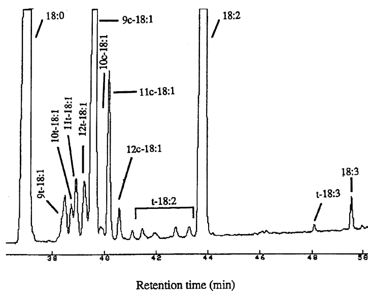
Figure 1 Separation of trans -18:1 positional isomers (as fatty acid methyl esters) of plasma phospholipid fatty acids separated using a 100 m BPX70 capillary column.
