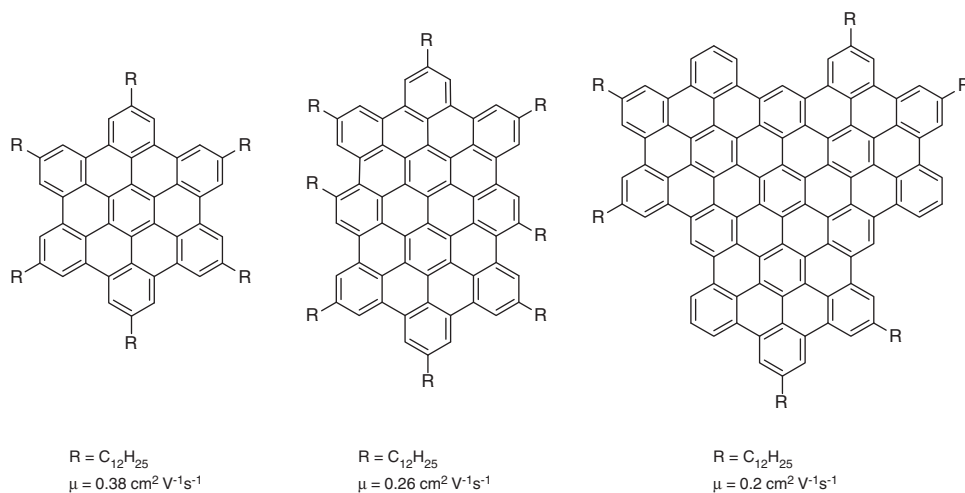
Figure 3 Some large core discotic liquid crystals with high charge carrier mobility.
