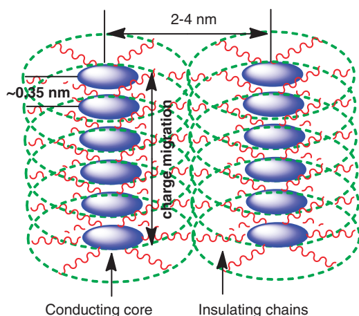
Figure 2 Representation of a columnar mesophase as a quasi-one-dimensional conducting system.
