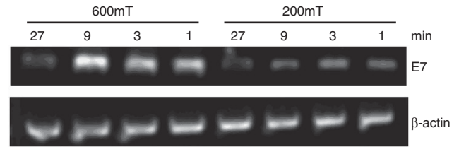
Figure 3. Semi-quantitative RT-PCR analysis of B16F10 cells transfected with BMP-V using various magnets and time periods. The expression was measured 48 h after transfection.
