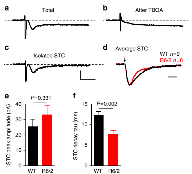
Figure 6 | Synaptically activated currents decay faster in R6/2 astrocytes. (a) Representative synaptically activated transporter current (STC) recorded in a striatal astrocyte, evoked by local electrical stimulation of glutamatergic afferents. The isolated STC (c) was obtained by subtracting the response in the presence of TBOA (100 μM, b) from that before TBOA application (a). Scale bars, 20 pA, 20 ms. (d) Average of all the isolated STCs recorded from WT (black, n = 9) and R6/2 (red, n = 8) astrocytes. The peaks are scaled for direct comparisons of the decay kinetics. Scale bar, 10 ms (e) Bar graph showing no difference in the average size of the isolated STCs (unpaired t-test). (f) Bar graph showing a significant reduction in the decay time of STCs recorded from R6/2 astrocytes (unpaired t-test).
