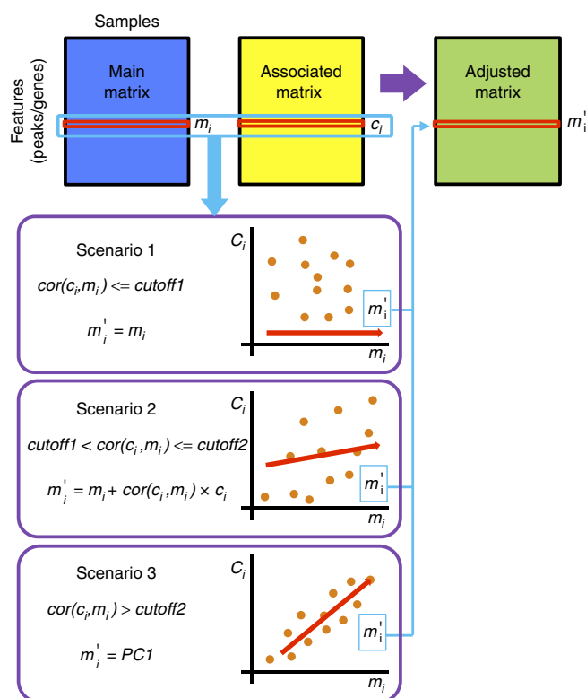
Figure 1 | Overview of MANCIE. Each row vector in the adjusted matrix is generated from the corresponding row vectors in the main matrix and the associated matrix. On the basis of the correlation between the main row vector m_i and the associated row vector c_i , one of three scenarios will be chosen. See more details in the online methods.
