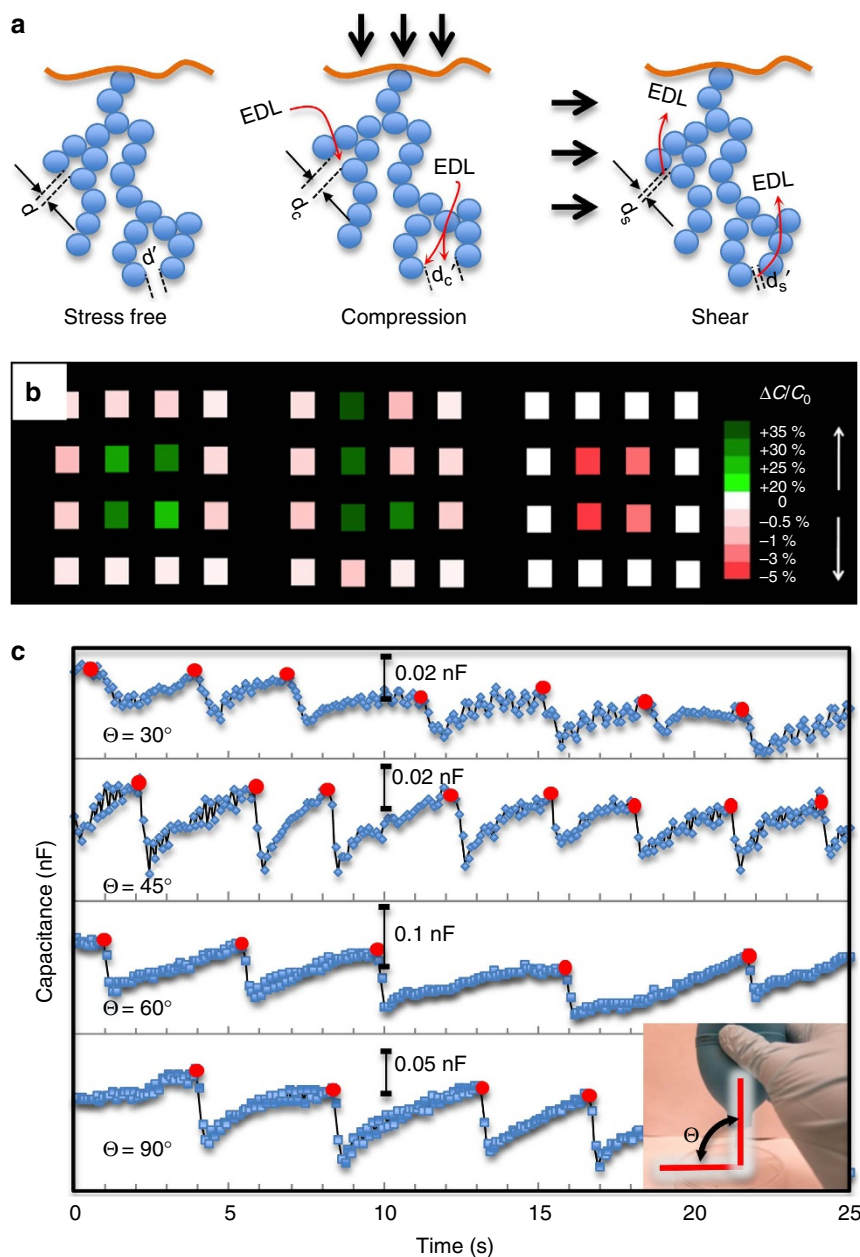
Figure 3 | Response of hydrogel capacitors to deformations in air. (a) Deformable network of metal nanoparticles (MNPs) makes the hydrogel sensitive to external load: (stress free) MNP network has fractal branches not yet wide open for EDL (electric double layer) build-up; (Compression) vertical pressure separates fractal branches apart ( d_c > d and d_c' > d' ), promoting charge trapping (increased capacitance due to EDL insertion); and (shear) lateral pressure squeezes branches together ( d_s < d and d_s' < d' ), closing gaps for EDL (reduced capacitance). (b) Array of MNP in the hydrogel can be used to map out contour of shaped loads of 8.0 kPa, from left to right for the shape of an 'O', an 'L' and a small dot. Capacitance increases (green; arrow up) or decreases (red; arrow down) due to location of the loads. (c) Angle-dependent sensing of airflows (red dot) suggests shear-induced pore closing in MNP for capacitance reduction. Inset photo illustrates the airflow angle ( \Theta ).
