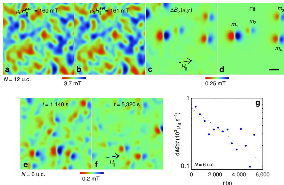
Figure 2 | Field-driven and temporal magnetization reversal dynamics in LMO/STO. (a,b) Two consecutive 1.5 \times 1.5 \mu\text{m}^2 images of B_z(x, y) (see Supplementary Movie 2) in an N = 12 u.c. sample after a field excursion to \mu_0 H_{||}^{\text{set}} = 160 (a) and 161 mT (b). (c) Differential image \Delta B_z(x, y) obtained by direct subtraction of (a) from (b) revealing magnetization reversal events of isolated SPM nanoscale islands (see Supplementary Movie 3). Note an order of magnitude enhanced colour scale. (d) Numerical fit to \Delta B_z(x, y) in (c) with four in-plane oriented islands using SOT diameter of 104 nm, scan height of 105 nm, and N_e = 2 u.c. with resulting magnetic moments m_1 = 1.0 \times 10^5 \mu_B ( D_1 = 40 nm), m_2 = 2.6 \times 10^4 \mu_B ( D_2 = 20 nm), m_3 = 4.7 \times 10^4 \mu_B ( D_3 = 28 nm), and m_4 = 6.8 \times 10^4 \mu_B ( D_4 = 33 nm). Scale bar is 200 nm. (e) B_z(x, y) image in N = 6 u.c. sample showing the thermally activated magnetization reversals of the islands at a constant \mu_0 H_{||} = 80 mT at t = 1,140 s after the field ramp (see Supplementary Movie 6). (f) Same as (e) at t = 5,320 s. (g) The magnetization relaxation rate dM/dt attained by vectorial summation of the reversal events m in each frame of Supplementary Movie 6. Dotted line is a guide to the eye.
