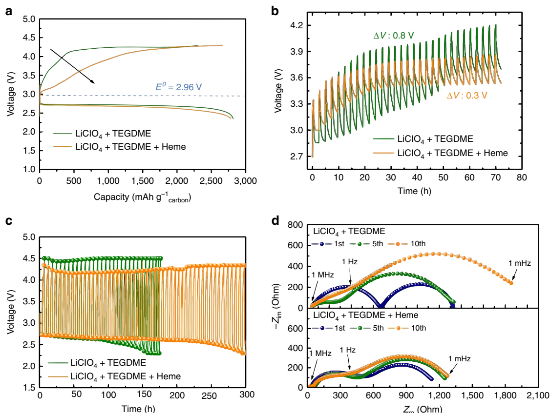
Figure 2 | Li-O 2 cell performance in heme-containing electrolyte. (a) Initial charge/discharge curves of the MWCNT electrode in 1 M LiClO 4 + TEGDME and 1 M LiClO 4 + TEGDME + Heme solutions in a voltage window between 4.3 and 2.35 V at a current density of 100 mA g -1 carbon; (b) galvanostatic intermittent titration curves of the MWCNT electrode in 1 M LiClO 4 + TEGDME and 1 M LiClO 4 + TEGDME + Heme solutions, which were acquired with a current density of 50 mA g -1 for 24 min and a 120 min time interval during the 1st charging; (c) Voltage versus time curves of the MWCNT electrodes in 1 M LiClO 4 + TEGDME + Heme solution at various cycles under a specific capacity limit of 600 mAh g -1 between 4.5 and 2.3 V at a current density of 200 mA g -1 carbon; (d) Electrochemical impedance spectroscopy (EIS) spectra of the MWCNT electrode in 1 M LiClO 4 + TEGDME and 1 M LiClO 4 + TEGDME + Heme solutions after the 1st, 5th, and 10th discharge cycle.
