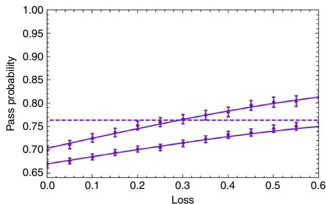
Figure 4 | Impact of noise and loss on the pass probability of the \theta -verification protocol in a four-party setting.
