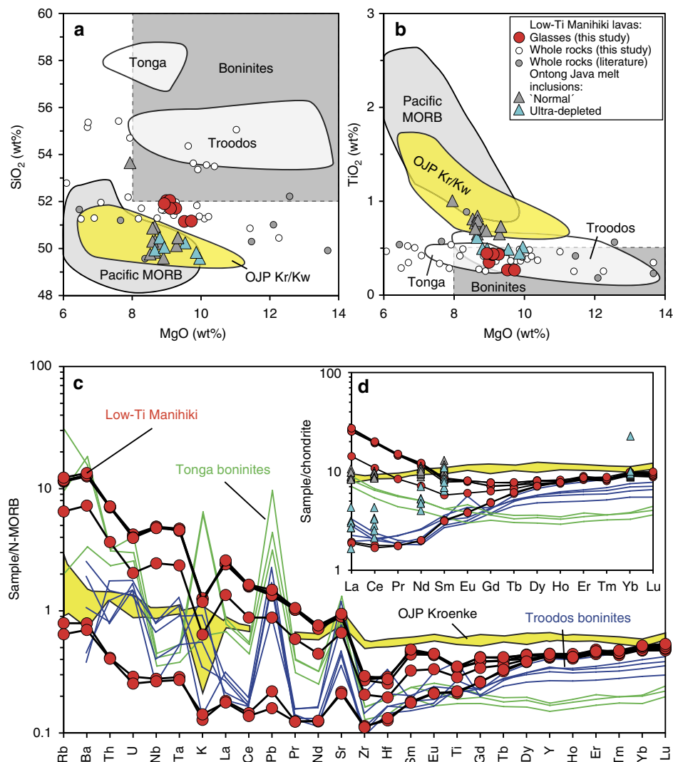
Figure 2 | Selected major oxide and incompatible element compositions of low-Ti Manihiki rocks and glasses. (a) \text{MgO} versus \text{SiO}_2 and (b) \text{MgO} versus \text{TiO}_2 plots for low-Ti Manihiki glasses (red circles) and whole rock samples (white circles: this study, Supplementary Table 2; grey circles: data from refs 4,13). All major element oxide data were normalized on a volatile-free basis to 100%. Compositional fields for Tonga and Troodos boninites 26,27 , Kroenke/Kwaimbaita OJP rocks and glasses 6,15 , melt inclusions from Ontong Java 16 and Pacific MORB 66 are shown for reference. Compositional range of boninites ( >52 wt% \text{SiO}_2 , >8 wt% \text{MgO} and <0.5 wt% \text{TiO}_2 ) is shown by grey field with dashed outer line 14 . (c) Incompatible element contents in low-Ti Manihiki glasses (black patterns), high-Ca boninites from Tonga (green patterns) and Troodos (blue patterns) normalized to N-MORB. (d) Rare earth elements in the same samples normalized to chondritic abundances. Most low-Ti glass samples from Manihiki have U-shaped patterns similar to boninites, reflecting in part re-enrichment of the most incompatible elements in a depleted source. Direct comparison of incompatible elements shows that boninite-like low-Ti Manihiki glasses do not show enrichment in fluid-mobile elements or negative Nb-Ta anomalies characteristic of boninites. Representative compositions for Troodos and Tonga boninites 67,68 and OJP Kroenke-type rocks (OJP Kroenke; yellow field) 6 are also shown. OJP inclusions 16 in d have similar labelling as in a,b. N-MORB and chondrite compositions for normalization are from ref. 32.
