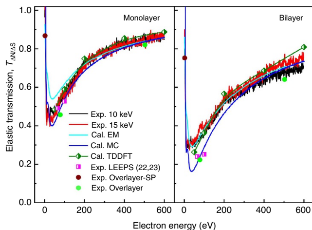
Figure 3 | Elastic transmission of mono- and bilayer graphene. Elastic transmission ( T_{\Delta N/\Delta S}(E) , that is J_{\Delta N}(E)/J_{\Delta S}(E) ) of monolayer graphene and bilayer graphene measured by the virtual substrate method for primary electron energies of 10 and 15 keV. The elastic transmission was calculated by the extended Mermin (EM), Monte Carlo (MC) and time-dependent density functional theory (TDDFT) methods. The total transmission was measured by low-energy electron point-source (LEEPS) microscopy 22,23 corrected to the elastic transmission by the MC method. The elastic transmission was measured by the overlayer method for graphene/gold at 2.3 eV, associated with gold surface plasmons (overlayer-SP), and for graphene/SiO 2 samples at 78 and 503 eV (overlayer).
