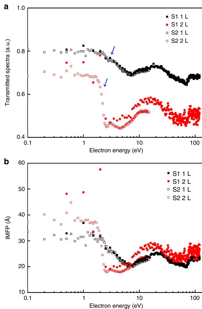
Figure 5 | Electronic properties of monolayer and bilayer MoS 2 .
