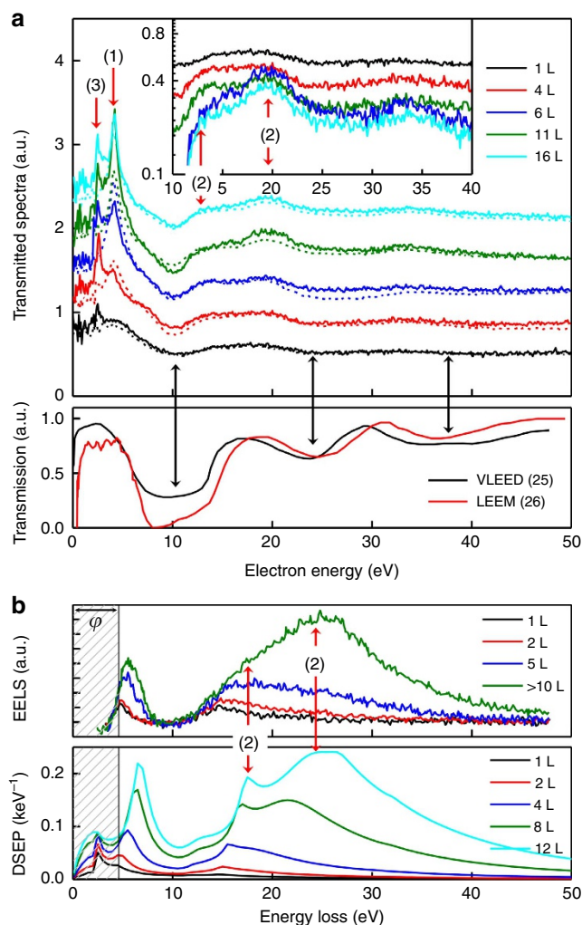
Figure 4 | Material characterization using the virtual substrate method.
