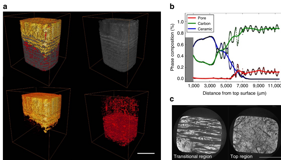
Figure 3 | Morphology of C/C- \text{Zr}_{0.8}\text{Ti}_{0.2}\text{C}_{0.74}\text{B}_{0.26} /SiC via X-ray computed-tomography. (a) Overall view of composites showing carbides (yellow), carbon fibres and pyrocarbon (grey) and pores (red). Due to the resolution limit, only pores larger than 1,000 \mu\text{m}^3 are quantified. (b) Distributions of the phases from the top to the bottom of the sample determined from the X-ray computed tomography (CT) virtual slices. The dots are the volume percentage of each phase calculated from each virtual slice. The solid lines are the fitted curves. The zig-zag shape of the dot is due to the alternating plies. The grey area represents the top of the sample which has been excluded from quantification due to strong artefacts. (c) Virtual CT cross-sections showing the transitional region comprising the carbon matrix and ceramic (40 vol. %) and a region near the top (ceramic: 76 vol. %). Scale bar, 5 mm.
