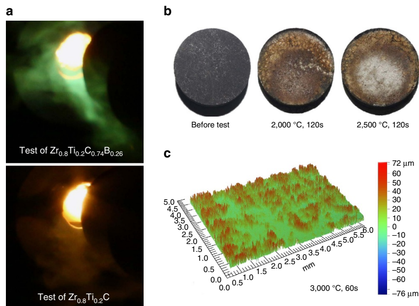
Figure 2 | Photograph of ablation test and morphology of tested sample. (a) Green and orange flames are seen in tests of \text{Zr}_{0.8}\text{Ti}_{0.2}\text{C}_{0.74}\text{B}_{0.26} and \text{Zr}_{0.8}\text{Ti}_{0.2}\text{C} , respectively. (b) Comparison of surface of the 30 mm diameter samples before and after ablation. Black-gray sample is before test, and middle and right samples experienced 120 s ablation of 2,000 °C and 2,500 °C, respectively. (c) Surface profile of central region of sample ablated at 3,000 °C, showing the ablated traces (some convexities with the rises of <72 \mu\text{m} ) due to evaporations of oxides with low melting points (see Protective mechanisms). But no ablated hollows appeared on surface.
