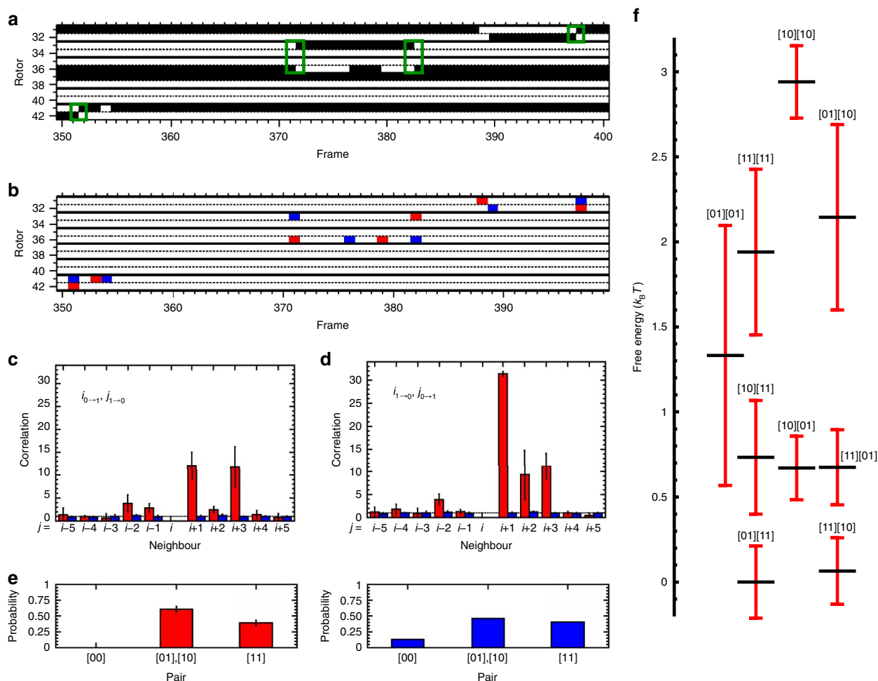
Figure 2 | Statistical analysis of correlated switching. (a) Example on/off trajectory of the major crystal at -10 mV and 10 pA. White and black denote ethyl rotors pointing up (on; 1) and down (off; 0), respectively. Correlated switches are highlighted by green boxes. (b) Corresponding switching trajectory. Blue and red denote switching off ( 1 \rightarrow 0 ) and switching on ( 0 \rightarrow 1 ), respectively. Statistical analysis of 1,724 events reveals non-random switching and the predominance of several correlated switching events. The correlations plotted here are (c), the ratio of the conditional probability of an ethyl rotor at position j ( j = i - 5, \dots, i - 1, i + 1, \dots, i + 5 ) switching off ( 1 \rightarrow 0 ), given that the ethyl rotor at position i switches on ( 0 \rightarrow 1 ), to the average probability of an ethyl rotor switching off ( 1 \rightarrow 0 ) and (d) the ratio of the conditional probability of an ethyl rotor at position j switching on ( 0 \rightarrow 1 ), given that the ethyl rotor at position i switches off ( 1 \rightarrow 0 ), to the average probability of an ethyl rotor switching on ( 0 \rightarrow 1 ). The relative position of j to i is defined so that i + 1 is the NN of rotor i , while i - 1 is the FN of rotor i . The red and blue bars are results from experiment and from simulation of random switches, respectively. (e) Histogram of experimentally observed populations of [00], [01][10] and [11] (left, red), compared to a binomial distribution calculated with an optimized off probability of 0.36275 (right, blue). (f) Free energies of the nine most populated [ab][cd] microstates. Error bars are the weighted s.d. Similar free energy diagram using three-pair microstates [ab][cd][ef] can be found in Supplementary Fig. 20.
