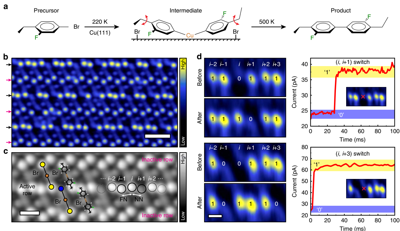
Figure 1 | Correlated switching in self-assembled molecular rotor crystals. (a) Surface-mediated Ullmann coupling reaction scheme. (b) STM image of a two-dimensional crystal composed of the reaction intermediate in which the ethyl rotors appear either as bright protrusions or depressions depending on their orientation. The reaction intermediates form an interlocked pattern and the ethyl rotors form active (exhibiting correlated switching; black arrows) and inactive rows (no switching; magenta arrows). Scale bar, 2 nm. (c) Zoom in of the active row with both colour-coded and molecular overlays. Yellow and blue circles indicate the up and down configurations of the ethyl rotors, respectively. An example of ethyl rotor indexing is shown where i+1 and i-1 denote the NN and FN of rotor i , respectively. Scale bar, 1 nm. (d) Same-pair ( i, i+1 ) and long-range ( i, i+3 )-correlated switching observed when pulsing rotor i in the active row with the STM tip. The resultant current versus time traces are shown with the location of the STM tip pulses ( \pm 50 mV) marked with a red cross; scale bar, 0.5 nm, and imaging performed at -10 mV and 5 pA.
