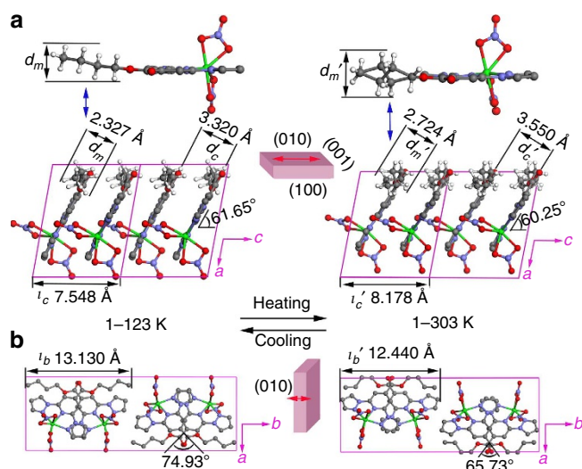
Figure 5 | Molecular packing of a crystal of 1. Crystalline packing of molecules of 1 in the low- and high-temperature phase ( 1 —123 K and 1 —303 K) as viewed from (a) the (010) face and (b) the (001) face. From the low-temperature phase to the high-temperature phase (a) the size of the n -butyl group in the direction perpendicular to the molecular plane ( d_m ), the average distance between the molecules along the c axis ( d_c ) and the length of the crystal c axis ( l_c ) increase to 2.724 Å ( d_m' ), 3.550 Å ( d_c' ) and 8.178 Å ( l_c' ), respectively; the tilt angle \varphi (Supplementary Fig. 2) decreases from 61.65 to 60.25° ( \varphi' , Supplementary Fig. 3); (b) the size of each molecular column decreases from 13.130 to 12.440 Å ( l_b \rightarrow l_b' ) along the b axis; and the crossing angle \omega (Supplementary Fig. 2) decreases to 65.73° ( \omega' , Supplementary Fig. 3). The outlines of the crystal morphology and red arrows in the middle of the diagrams show the direction of contraction and expansion of the crystal, respectively. Green, Co; grey, C; white, H; blue, N; red, O.
