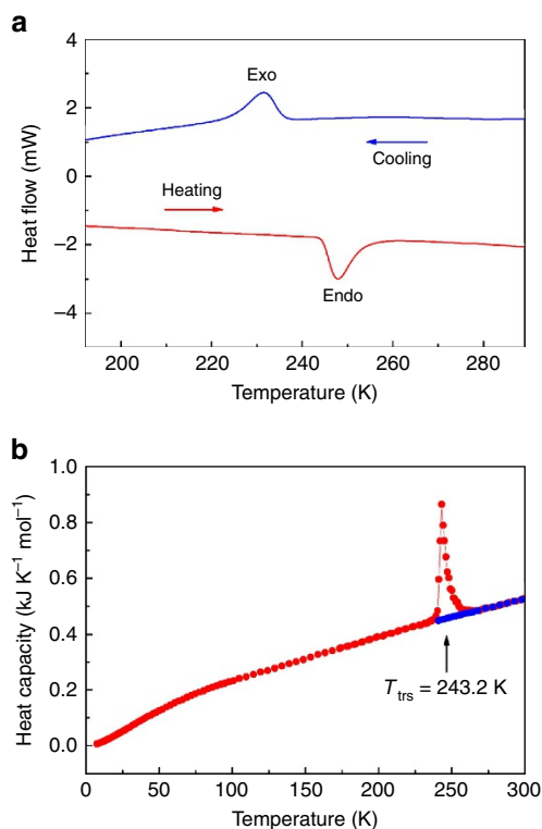
Figure 1 | Temperature dependence of differential scanning calorimetry and heat capacity for 1. (a) DSC curves of crystal 1 recorded at the rate of 10 K min −1 during a cooling–heating (blue–red lines) cycle. Exo: exothermic peak; Endo: endothermic peak. (b) The phase transition temperature ( T trs ) is determined to be 243.2 K on heating. Filled red and blue circles represent the data obtained during heating mode after the samples were cooled to 7.6 and 240.9 K, respectively.
