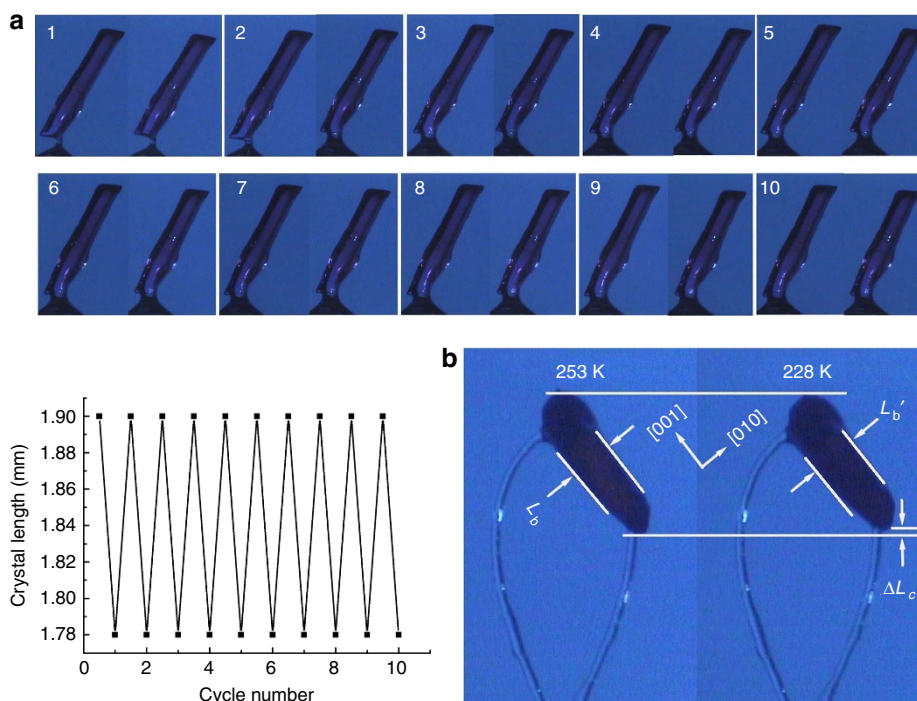
Figure 4 | Reversible shrinkage and expansion of crystal 1. (a) Reversible shrinkage and expansion of the prismatic crystal on alternate heating and cooling at a rate of 5 \text{ K min}^{-1} in the range 228–253 K. The crystal was glued onto a nylon loop and enveloped in a temperature-controlled stream of dry nitrogen gas. The crystal exhibits shrinkage and expansion along the long axis of the crystal in response to temperature. The reversible changes were recorded for 10 cycles without breaking the single-crystal state. (b) The increase in crystal size from \sim 0.20 ( L_b ) to 0.21 \text{ mm} ( L_b' ) along the [010] direction, and the contraction by \sim 0.05 \text{ mm} ( \Delta L_c ) (from about 0.83 to 0.78 \text{ mm} ) during cooling from 253 to 228 \text{ K} .
