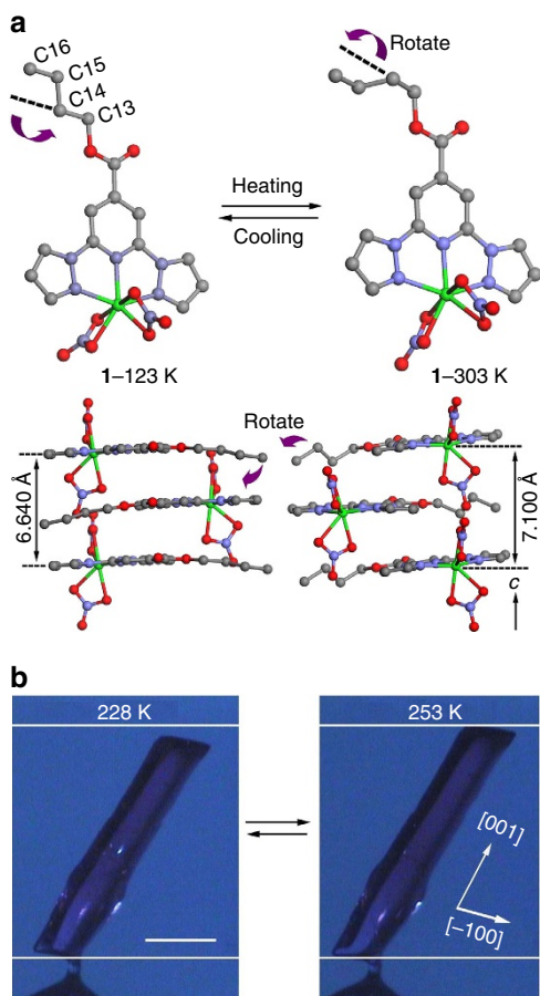
Figure 2 | Molecular structures of crystal 1 in the low- and high-temperature phase. (a) The cobalt ions are coordinated by one tripodal L ligand and two nitrate anions in both phases. The molecules stack in parallel along the c axis with different distances between molecules in the low- and high-temperature phases. The n -butyl group of the ligand rotates ca. 100° around the C13–C14 bond following phase transition. Green, Co; grey, C; blue, N; red, O. Hydrogen and disordered carbon atoms (C14' and C15') are omitted for clarity. (b) The crystal length changes from 1.78 to 1.90 mm along [001] from 228 to 253 K and switches back to the original state upon cooling, scale bar represents 500 μm.
