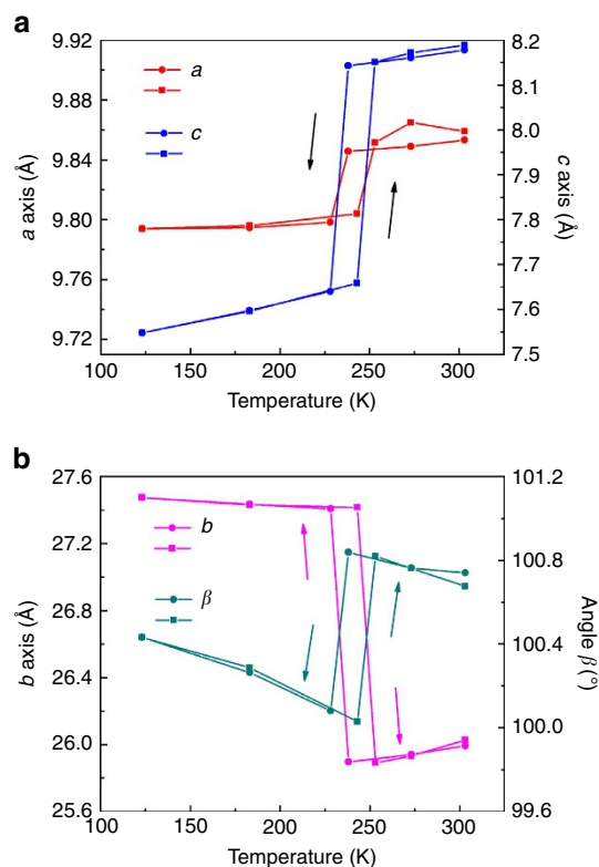
Figure 3 | Cell metrics as a function of temperature. Variable-temperature single-crystal X-ray diffraction data of complex 1 were repeatedly collected for the same crystal in the range 123–303 K (heating, filled squares; cooling, filled circles). (a) Changes in the crystallographic a and c axes. (b) Variations of the angle \beta and the crystallographic b axis. The length of the b and c axes exhibit a reversible and abrupt change at ~240 K and the percentage change is ~5, respectively.
