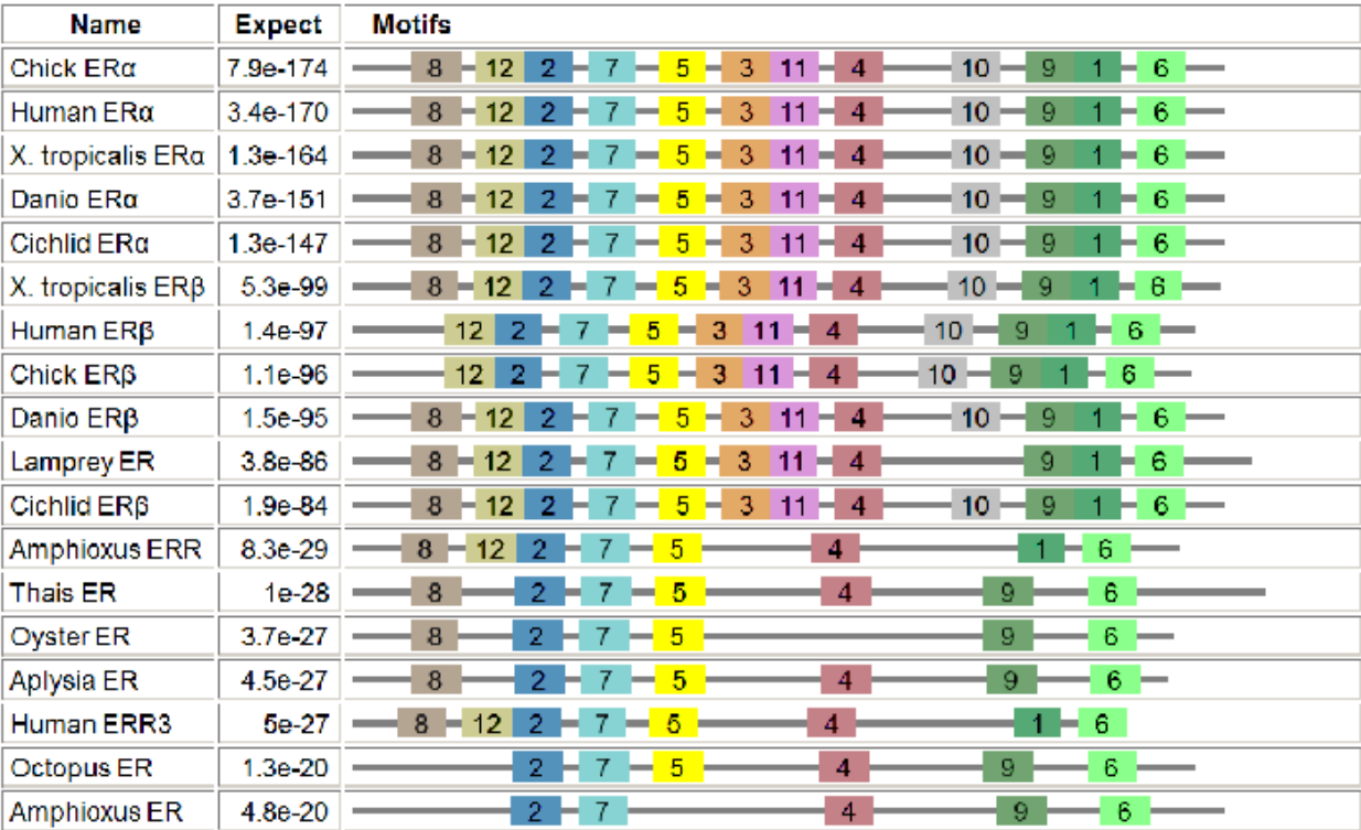
Figure 2. MAST analysis of MEME motifs for the ERα training set
