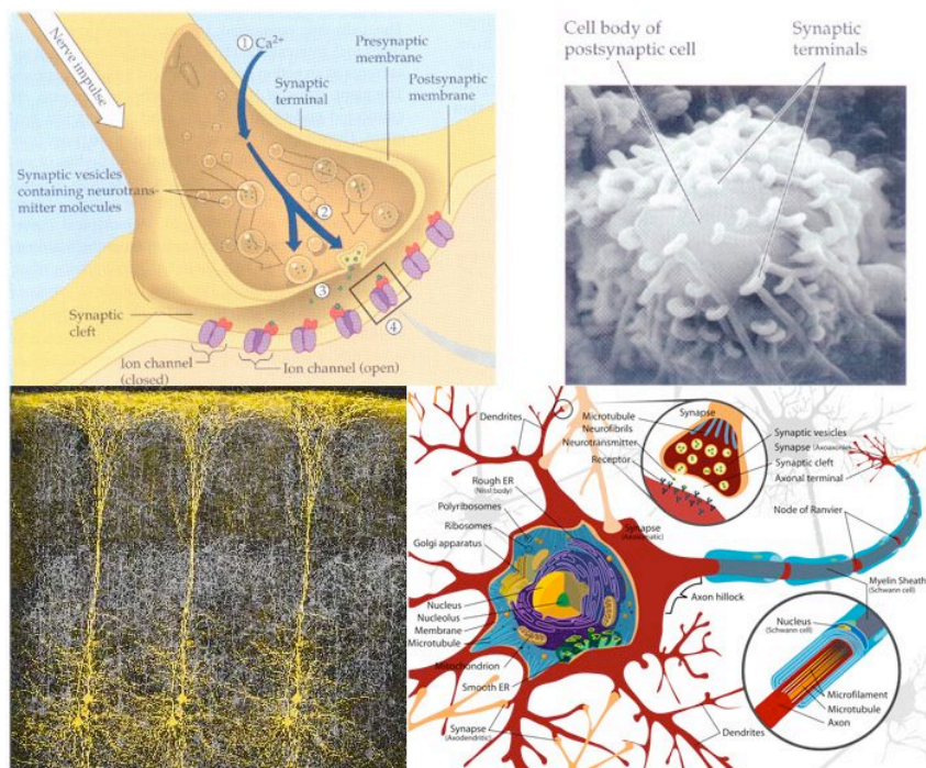
Fig 4: Quantum fractality differs from classical fractality in that it becomes discrete at the quantum level. Fractal scale transformations emerge from quantum non-linearities forming the chemical bond, in emergent stages through tertiary and quaternary molecular structures, to cellular organelles, cells, tissues and finally the whole organism, with its successive bifurcations of development to form the tissue layers and later, interactive migrations of specific cell types. Nervous system organization is thus fractal, running from the molecular level of ion-channels, to neurotransmitter vesicles and synaptic junctions (upper), then to neurons (lower right), then to neuronal complexes such as mini-columns (lower left) and finally to whole brain activation.
