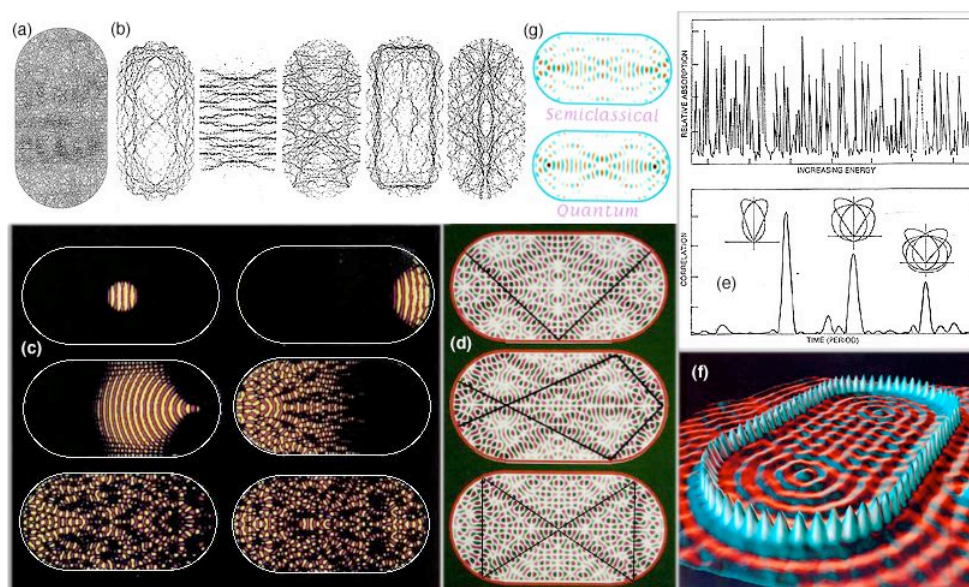
Fig 8: Quantum chaos: The classical stadium billiards is chaotic. A given trajectory has sensitive dependence on initial conditions. As well as space-filling chaotic orbits (a) 39 , the stadium is densely filled with repelling periodic orbits, three of which are shown in black in (d). Because they are repelling, neighbouring orbits are thrown further away, rather than being attracted into a stable periodic orbit, so arbitrary small deviations lead to a chaotic orbit, causing almost all orbits to be chaotic. The quantum solution of the stadium potential well (b) 40 and (d) 41 shows 'scarring' of the wave function along these repelling orbits, thus repressing the classical chaos, through probabilities clumping on the repelling orbits. A semi-classical simulation (c) shows why this is so. A small wavelet bounces back and forth, forming a periodic wave pattern, because even when slightly off the repelling orbit the wave still overlaps itself and can form standing wave constructive interference when its energy and frequency corresponds to one of the eigenvalues of a periodic orbit, even though the orbit is classically repelling. The quantum solution is scarred on precisely these orbits (d). This causes resonances such as absorption peaks of a highly magnetically excited atom (e) to coincide with the eigenfunctions of the repelling periodic orbits, just as the orbital waves of an atom constructively interfere with themselves, in completing an orbit to form a standing wave, like that of a plucked string. The result is that, over time, in the quantum system, although the behaviour may be transiently chaotic, it eventually settles into a periodic solution. Experimental realizations such as the scanning tunneling view of an electron on a copper sheet bounded by a stadium of carefully-placed iron atoms (f) 42 , confirm the general picture, although, in this experiment, tunneling leaked the wave function outside too much to demonstrate proper scarring. The semi-classical approach matches closely to the full quantum calculation (g).
