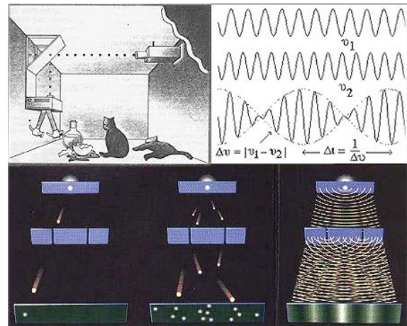
Fig 7: Top right: Beats of constructive wave interference determine the uncertainty principle. Bottom: Two-slit interference experiment illustrates wave-particle complementarity. Top left: Cat Paradox experiment.
