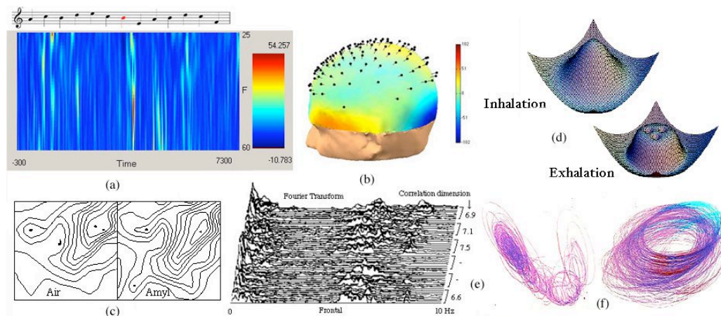
Fig 2: Evidence for both dynamical chaos and phase wave-front 'holographic' processing. (a) Wavelet (morlet) transform, showing time evolution of amplitudes with a peak in the gamma band accompanying recognition of an anomalous note is consistent with phase-front processing. Broad-spectrum excitation (extended vertical distribution of frequencies) is also consistent with chaotic dynamics in the time domain. (b) Coherent distribution of electroencephalogram over the cortex, is consistent with globally coupled excitation. (c) Extended spatial distribution of cortical activation accompanying recognition of an odour. (d) Freeman's 16 17 model of olfactory recognition involves a transition from high-energy chaos on inhalation to enter a new or existing strange attractor basin as the energy is lowered on exhalation. Although this is a transition from chaos to an ordered outcome, the attractor may be a strange attractor, still supporting chaos locally within the basin. (e) Fourier transforms of electroencephalogram, showing broad-spectrum excitation and correlations dimensions consistent with global chaotic dynamics. (f) Putative strange attractors in the electroencephalogram.
