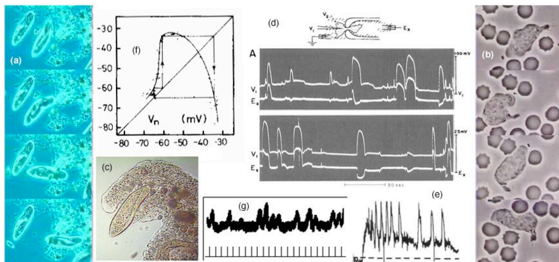
Fig 9: Real-time purposive behavior in single cells (a) Paramecium reverses, turns right and explores a cul-de-sac. (b) Human neutrophil chases an escaping bacterium (black), before engulfing it. (c) Chaos chaos engulfs a paramecium . Action potentials in Chaos chaos (d) and paramecium (e). Period 3 perturbed excitations in Nitella confirm chaos. (g) Frog retinal rod cells are sensitive to single quanta in an ultra-low intensity beam, with an average rate of one photon per click, but sometimes zero, or two, due to uncertainty in the beam.
