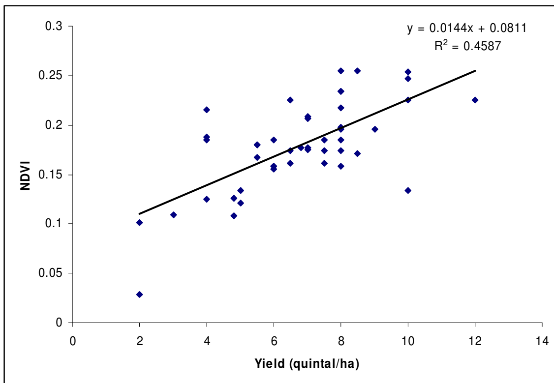
Figure.4.A regression analysis was performed to verify that how NDVI was able to predict the yield and it was found that a good correlation (0.697) existed between the NDVI yield and the R^2 value was also found to be very significant (0.4587).
