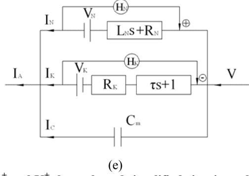
Fig.3 The equivalent circuits for \text{Na}^+ and \text{K}^+ channels and simplified circuit model for action potential (a) equivalent circuit for \text{Na}^+ channel (b) equivalent circuit for \text{K}^+ channel (c) simplified equivalent circuit for \text{Na}^+ channel (d) simplified equivalent circuit for \text{K}^+ channel (e) simplified circuit model for action potential
