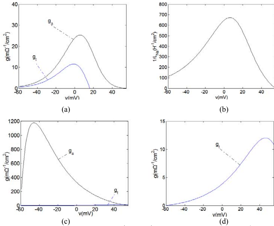
Fig.4 The electrochemical impedances of the \text{Na}^+ and \text{K}^+ channels (a) g_t and g_a for \text{Na}^+ channel (b) L_N for \text{Na}^+ channel (c) g_t and g_a for \text{K}^+ channel (d) g_t for \text{K}^+ channel
