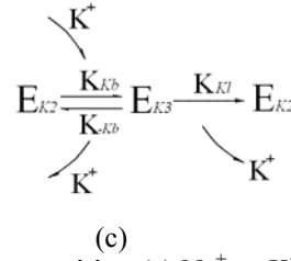
Fig.1 Na + and K + channels, and their kinetic models for state transition (a) Na + or K + channel, (b) kinetic model for Na + channel, (c) kinetic model for K + channel
