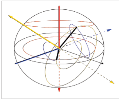
Paths taken by vectors in the Poincaré sphere under birefringence. The propagation modes (rotation axes) are shown with red, blue, and yellow lines, the initial vectors by thick black lines, and the paths they take by colored ellipses (which represent circles in three dimensions).
