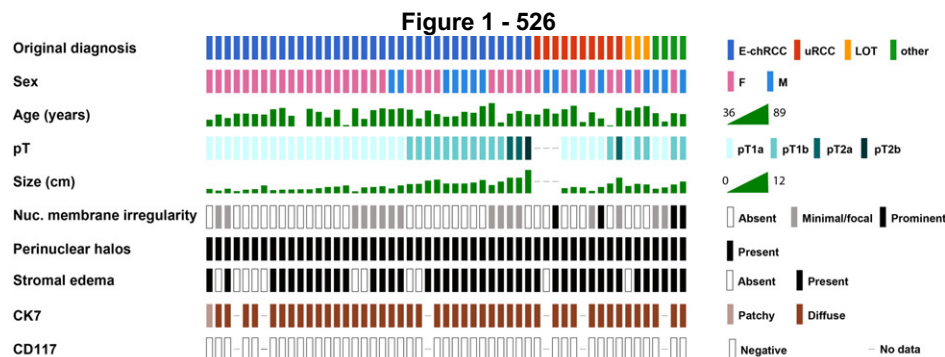
Figure 1. Clinical, morphologic, and immunohistochemical features of 53 low-grade oncocyctic tumors (LOT). E-chRCC: eosinophilic variant of chromophobe renal cell carcinoma; uRCC: unclassified renal cell carcinoma.
