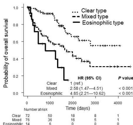
Figure 2: Kaplan-Meier curve of overall survival (TCGA cohort)
