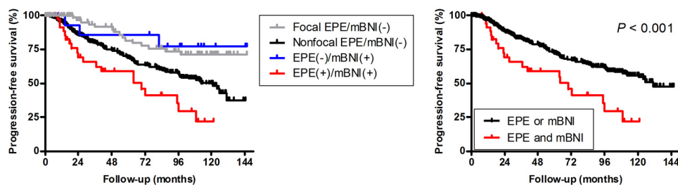
Figure 1. Progression-free survival in all patients.
