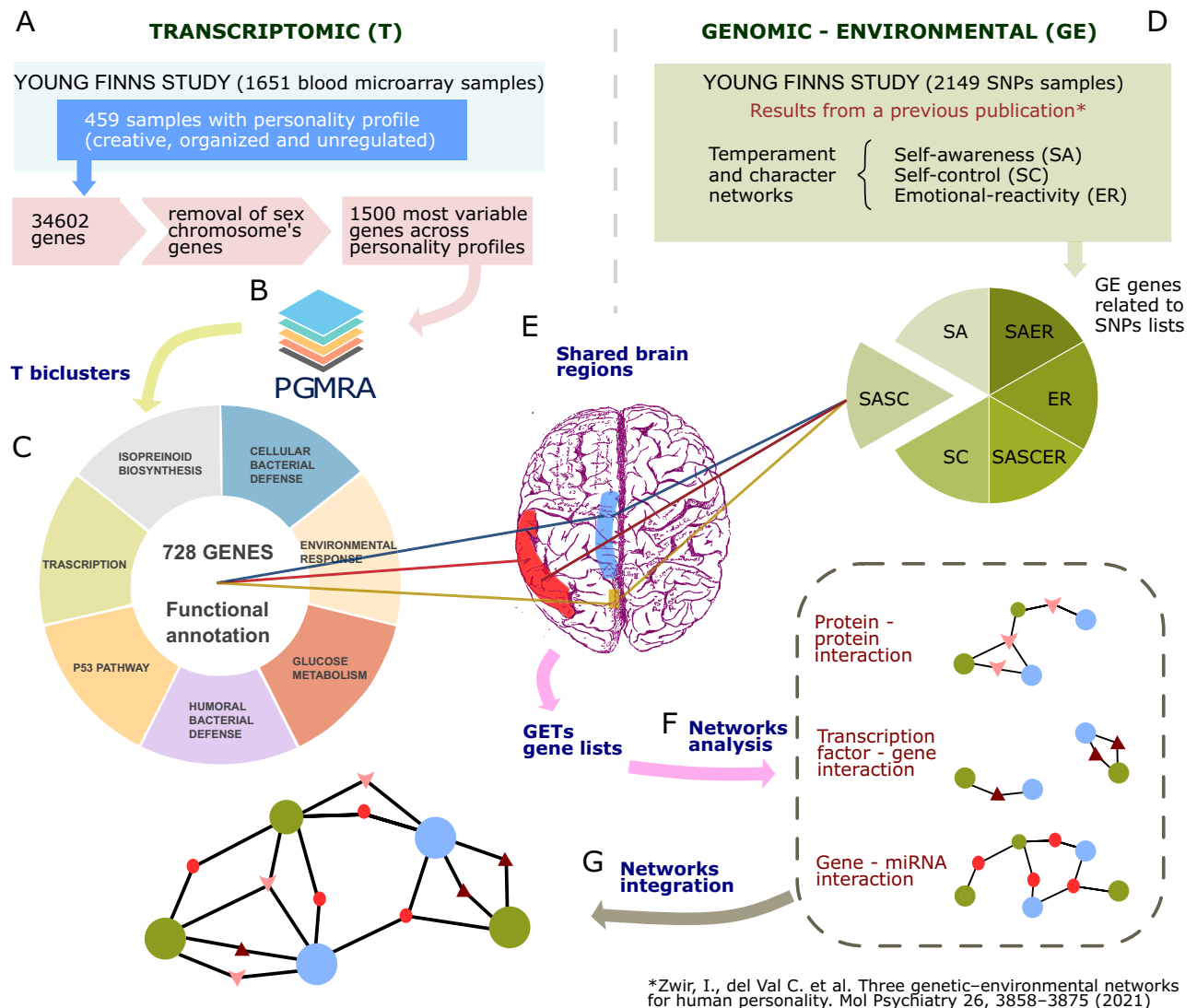
Fig. 1 Methodology flowchart. A Transcriptomic (T) data processing workflow. B PGMRA analysis on T data and T- biclusters generation. C Functional annotation of PGMRA T-biclusters. D Collection of gene sets from the three Genomic-Environmental networks (GE) of human personality from Zwir et al. 2021. E Mapping of the T-biclusters and GE gene sets to brain regions, specifying GET gene subsets. F GET biological interaction analysis with three types of interaction networks (protein-protein, transcription factors-genes and gene-miRNA) *. G Integration of interactions networks for each GET *. *Node colors distinguish transcriptomic genes (blue), genomic-environmental genes (green), and newly introduced genes by the type of bioinformatic network analysis (red). Node shape indicates the molecular subtype for the new genes from network analysis: triangle (protein), star (TF), and circle (miRNA).
