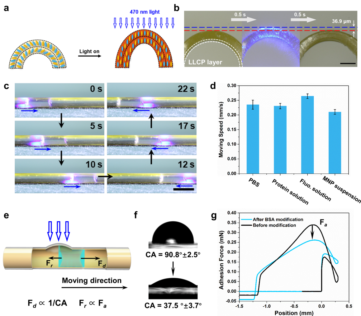
Fig. 2 Characterization of the PTM. a Schematic diagram showing the mechanism of LLC layer deformation upon irradiation with 470 nm light. b Photographs showing local radial expansion of the PTM cross section before and after irradiation with 470 nm light (80 mW cm -2 ). When the light is switched on, the PTM generates local expansion radially. As a consequence, the exposed surface of the PTM displaces upward 36.9 μm. After continuous illumination for 0.5 s, the displacement of the exposed surface reaches the maximum value. When the light is switched off, the displacement recovers within 0.5 s. The rapid recovery of the PTM is mainly due to the entropic restoring force of exposed regions and the elastic recovery of unexposed regions. Scale bar: 100 μm. c Photographs showing the photocontrolled motion of a protein droplet in the PTM. The intensity of the 470 nm light is 80 mW cm -2 . Scale bar: 2 mm. d Velocities of various reagent solution droplets, including phosphate buffered saline (PBS), protein solution, fluorescence solution, and magnetic nanoparticle (MNP) suspension, used during protein analysis in the PTM. e Schematic representation of the force analysis during the photocontrolled motion of droplets in the PTM, where F_d is the driving force, F_r is the resistance force, F_a is the adhesion force, and CA is the contact angle. f CAs of a 3 μL PBS droplet on the inner wall of the PTM before (top) and after (bottom) BSA modification. g Adhesion force curves of a 3 μL PBS droplet on the inner wall of the PTM before and after BSA modification. The maximum force decreases from 0.339 ± 0.031 mN (black) to 0.259 ± 0.043 mN (blue).
