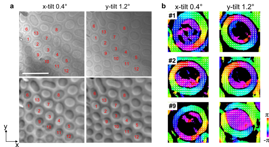
Fig. 2 | Real-space observation of field-free room temperature skyrmion bubbles after FC manipulation. a The 300 \mu\text{m} overfocused images (first row) and TIE retrieved phase images (second row) with an x-tilt of 0.4^\circ and a y-tilt of 1.2^\circ , respectively. The scale bar is 500 nm. b The configuration of the in-plane magnetic
