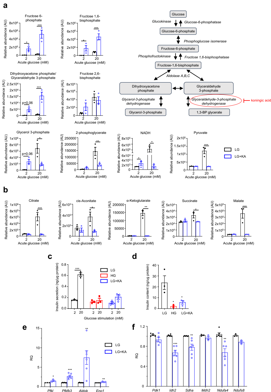
Fig. 4 | Inhibition of GAPDH induces changes similar to those caused by chronic hyperglycaemia. a Schematic of glycolysis showing where Koningic acid acts.
