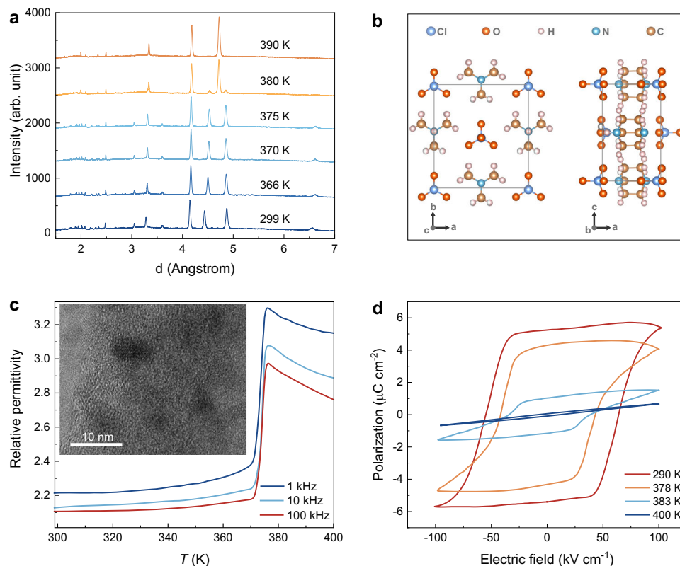
Fig. 2 | Structural and dielectric properties of energetic [Hdabco]ClO 4 .
