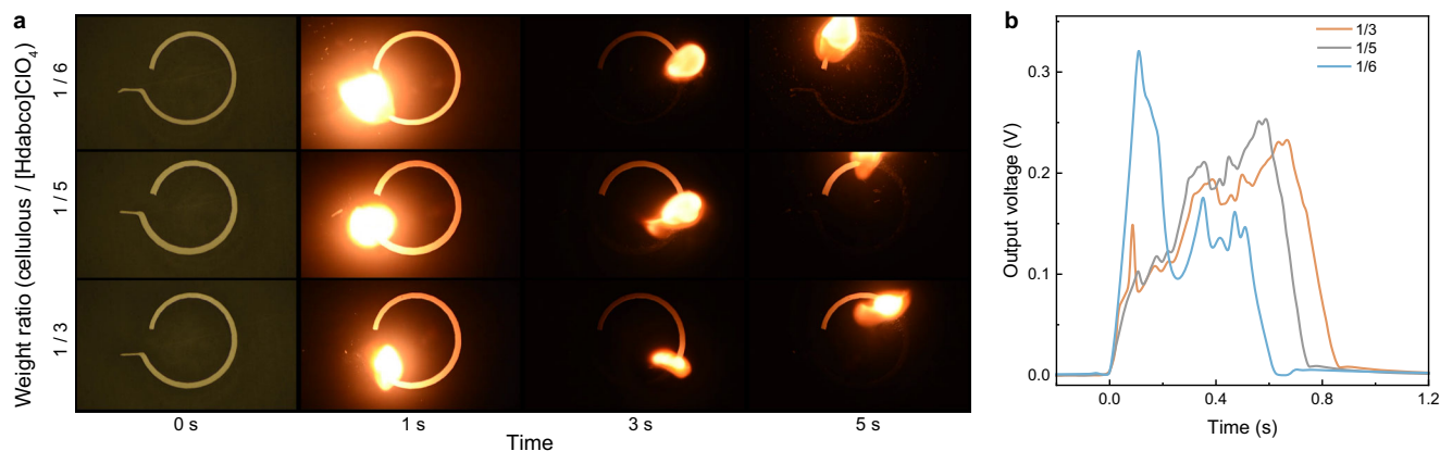
Fig. 6 | The control of chemical energy release. a , Selected snapshots from the video for the decomposition of 3D printed [Hdabco]ClO 4 with different weight ratios of cellulose/[Hdabco]ClO 4 . b , The decomposition generated electricity from [Hdabco]ClO 4 with different weight ratios of cellulose/[Hdabco]ClO 4 .
