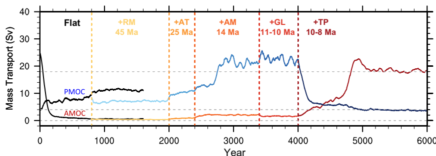
Fig. 1 | Temporal evolutions of the Atlantic meridional overturning circulation (AMOC) and Pacific meridional overturning circulation (PMOC) with the sequential uplift of different mountains in Flat2Real. The AMOC is represented by a red-scale colored curve, and the PMOC, by a blue-scale colored curve. Each segment corresponds to one mountain uplift. The “+” sign is used to indicate that a topography is added to the previous stage. The AMOC and PMOC indexes are
