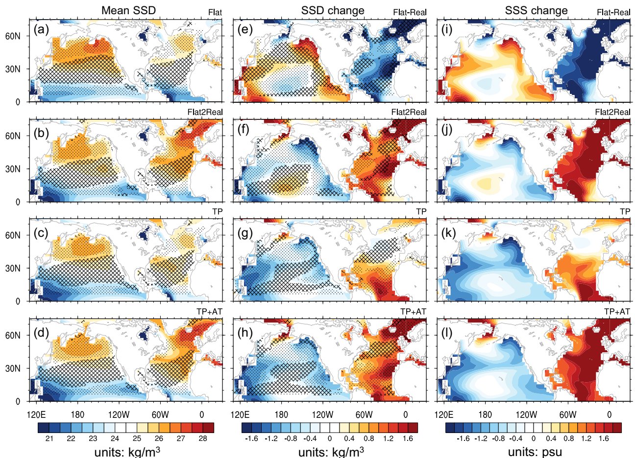
Fig. 4 | Mean sea surface density (SSD), Ekman pumping, and their changes. a–d Mean SSD (units: \text{kg/m}^3 ) in Flat, Flat2Real, TP (Tibetan Plateau), and TP + AT (Antarctic), respectively, with black dots (crosses) denoting mean Ekman upwelling (downwelling) in each experiment. The Ekman pumping is calculated as \omega_E = \text{curl}(\frac{\tau}{\rho}) , where \tau is the surface wind stress with units of \text{dyn/cm}^2 , \rho is the density of sea water ( 1024 \text{ kg/m}^3 ), and f is Coriolis parameter with units of 1/\text{s} . e shows the equilibrium changes in SSD and Ekman pumping in Flat with respect to Real, while f–h show their equilibrium changes in Flat2Real (Year 5601–6000), TP,
