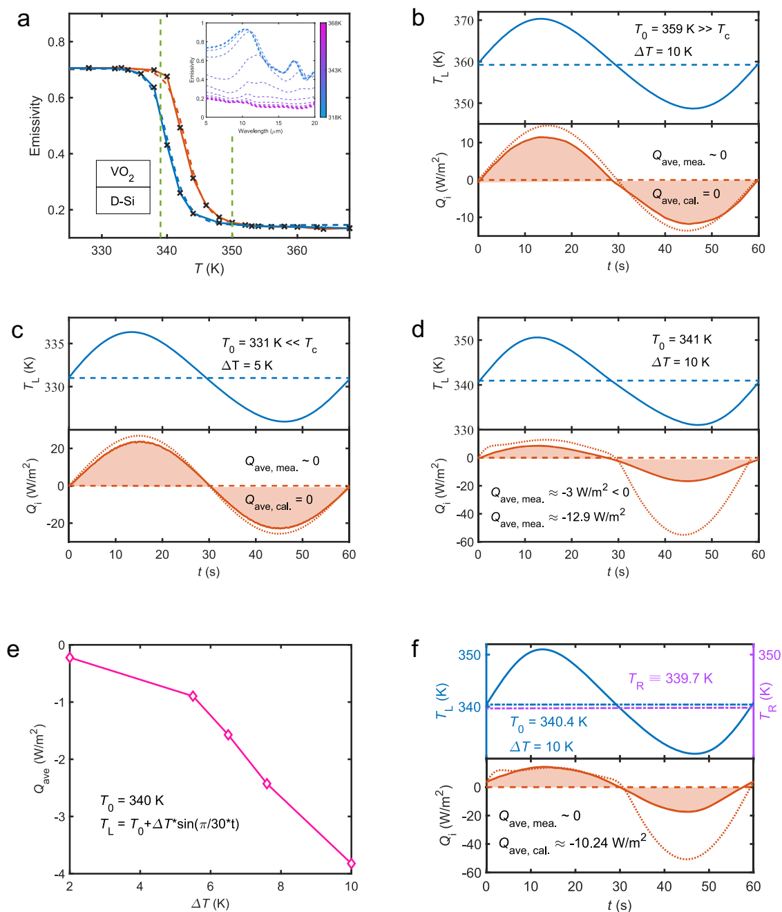
Fig. 2 | Heat shuttling effect in the backward scenario. a Emissivity of VO 2 (300 nm)/Si (200 \mu m) slab with respect to temperature during heating and cooling processes. Crosses correspond to experimental measurements. The inset gives the measured emissivity spectra at various temperatures. b–d Measured (solid line) and calculated (dotted line) temperature of the left slab and net heat flux between
