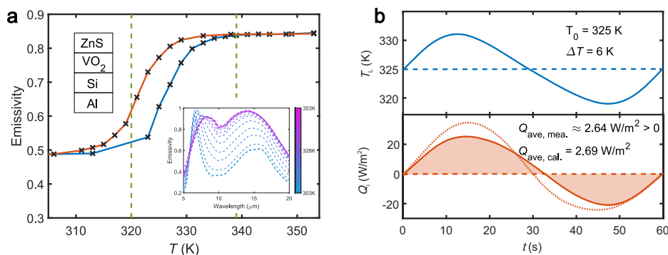
Fig. 3 | Heat shuttling effect in the forward scenario. a Emissivity of Al(130 nm)/Si(540 nm)/VO 2 (40 nm)/ZnS(1.08 μm)/Si(200 μm) slab with respect to temperature during heating and cooling processes. The inset gives the measured emissivity spectra at various temperatures. b Temperature variation of the left slab and
