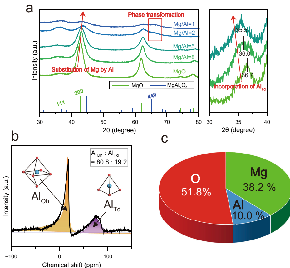
Fig. 1 | Structural characterizations. a XRD patterns obtained from Al-doped MgO samples having different Mg/Al ratios. Outset: an enlarged view of the MgO {111} region. b The 27 Al solid-state MAS-NMR spectrum acquired from a Ru/Al-MgO
