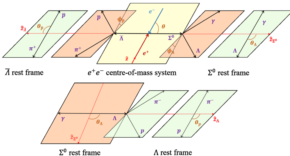
Fig. 2 | Definition of the helicity angles for J/\psi \rightarrow \bar{\Lambda}(\rightarrow \bar{p}\pi^+)\Sigma^0(\rightarrow \gamma\Lambda \rightarrow \gamma p\pi^-) . The angles \theta, \theta_{\Lambda}, \theta_p, \theta_{\bar{p}} are the polar helicity angles of the \Sigma^0, \Lambda, p and \bar{p} in the e^+e^- centre-of-mass system, \Sigma^0 rest frame, \Lambda rest frame and \bar{\Lambda} rest frame, respectively. The angles between different decay or production planes, \phi_{\Lambda} and \phi_{\bar{p}} , are the azimuthal helicity angles of the \Lambda and \bar{p} in the \Sigma^0 rest frame and \Lambda rest frame,
