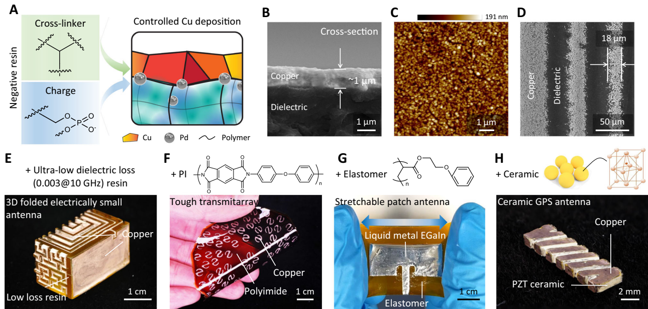
Fig. 2 | Optimization of selectivity and extension to other materials. A Schematic of the composition regulated copper deposition. B Scanning electron microscopic (SEM) image showing the cross section of copper cladding on the dielectric material. C Atomic force microscopic image showing the dense and smooth copper deposited on the negative resin. D SEM image showing the smallest feature size of CPD. E–H Demonstration of the enabled complex 3D antenna
