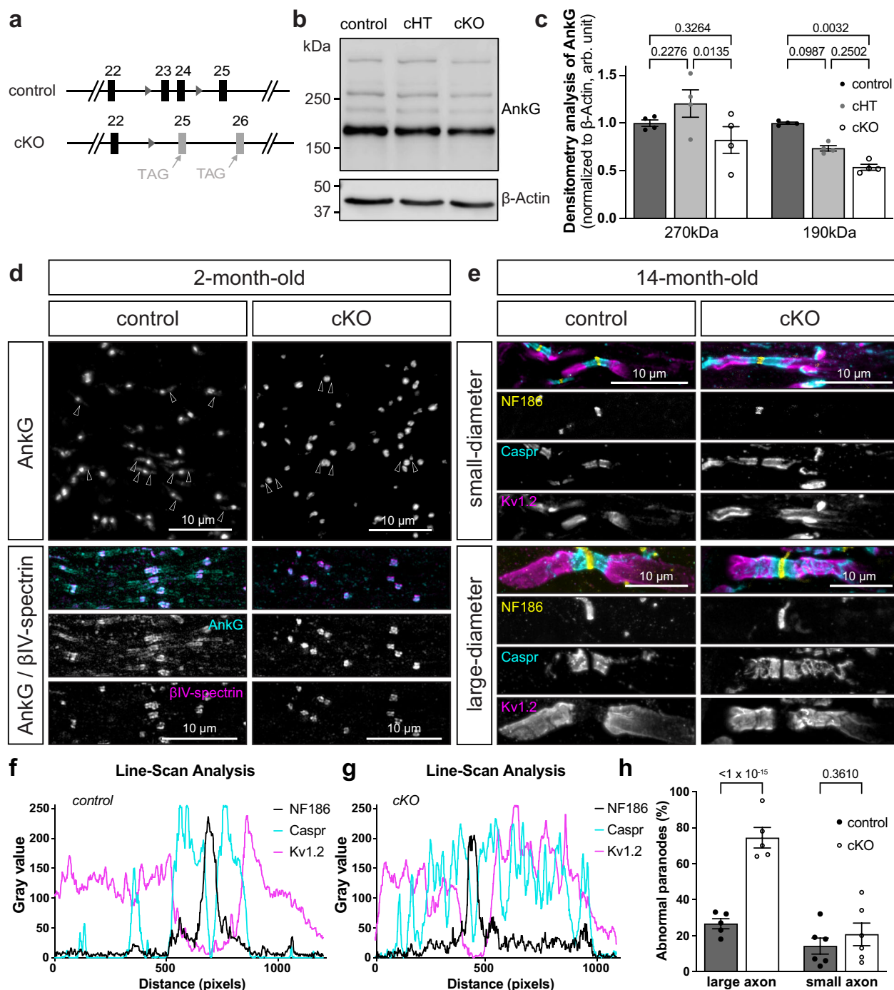
Fig. 1 | Loss of oligodendroglial AnkG leads to destabilization of paranodal junctions during aging. a Schematic of the Ank3 conditional allele and NG2 Cre -mediated recombination. b Immunoblot for AnkG in whole brain homogenates from 2-month-old control ( Ank3 f/f ), AnkG cHT ( NG2 Cre ; Ank3 f/f ), and AnkG cKO ( NG2 Cre ; Ank3 f/f ) animals. All three major isoforms of AnkG (480 kDa, 270 kDa, 190 kDa) are detected. \beta -Actin is the loading control. c Densitometry analysis of AnkG (270 and 190 kDa isoforms) in the brains of 2-month-old control, cHT, and cKO mice. N = 4 for each genotype. Two-way ANOVA with multiple comparisons. 270 kDa WT vs cHT: t = 2.423 , DF = 18.00 ; WT vs cKO: t = 2.084 , DF = 18.00 ; cHT vs cKO: t = 4.507 , DF = 18.00 . 190 kDa WT vs cHT: t = 3.108 , DF = 18.00 ; WT vs cKO: t = 5.445 , DF = 18.00 ; cHT vs cKO: t = 2.337 , DF = 18.00 . d Representative immunofluorescence staining of AnkG and \beta IV-spectrin in the optic nerve of 2-month-old control and cKO mice. Arrowheads indicate paranodes. Scale bar, 10 \mu m. (Cyan:
