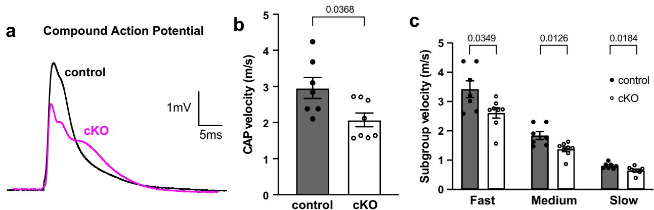
Fig. 4 | Loss of oligodendroglial AnkG results in slower conduction velocity of compound action potential. a Representative compound action potential (CAP) traces recorded from freshly dissected 14 month-old optic nerves with suction electrodes ex vivo. Black: control, Magenta: cKO. b The overall CAP velocity is calculated using the following formula: V_{CAP} = \text{Length of optic nerve} / (T_{Vmax} - T_{VO}) . N = 7 for control, N = 8 for cKO. Mann-Whitney test, two-tailed. U = 10 . c Three Gaussian curves are fitted under each trace to differentiate fast-, medium- and
