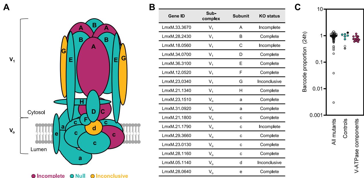
Fig. 6 | L. mexicana V-ATPase mutants are viable as promastigotes. A Schematic of V-ATPase subunits identified in L. mexicana , coloured by the genotype of the corresponding mutants. B Gene IDs of L. mexicana V-ATPase subunits. C Barcode proportions of mutants after 24 h of exponential growth in culture. Mutants were grouped into the following categories: ‘All mutants’ represent all non-V-ATPase transporter mutants in the pool (dark grey dots); ‘Controls’ represent the barcoded
