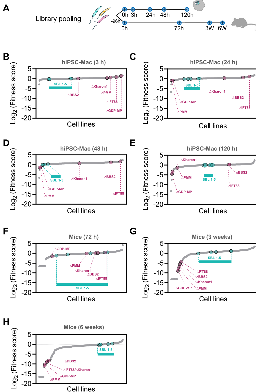
Fig. 4 | Fitness of intracellular Leishmania , in macrophages and in mice.
