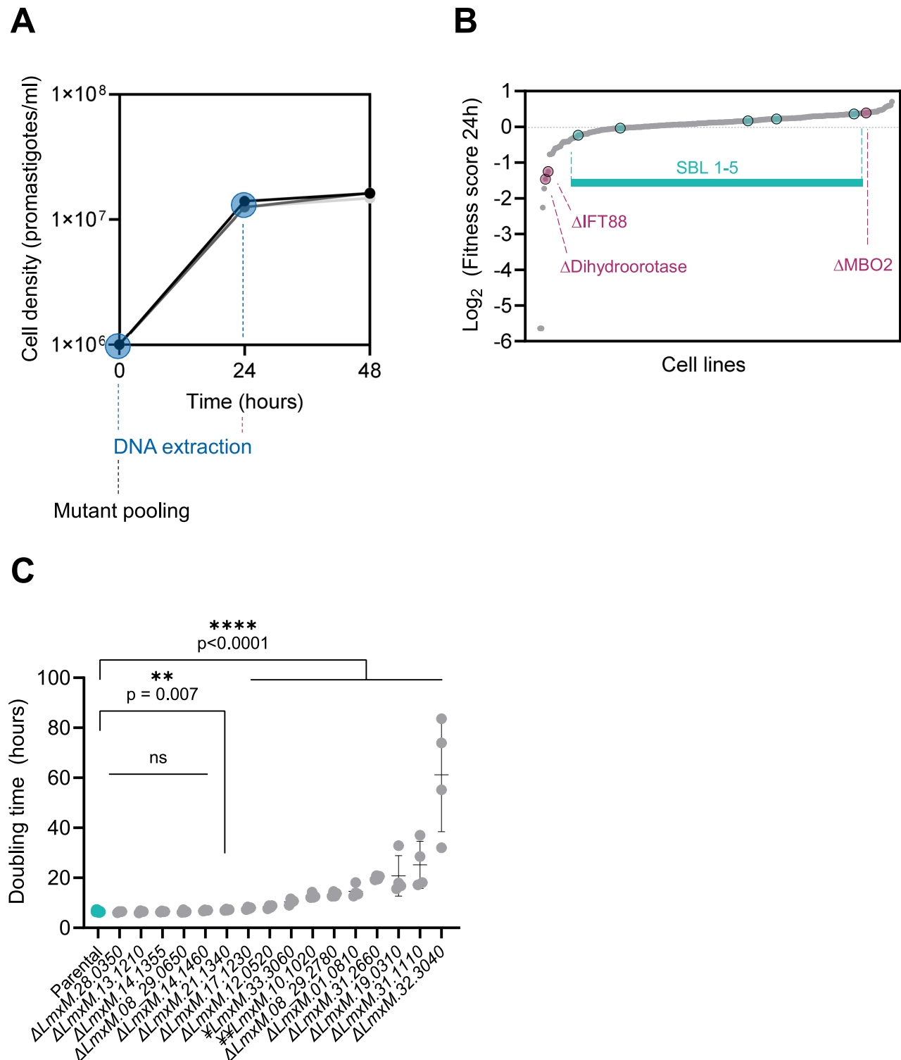
Fig. 3 | Fitness of promastigote mutants in vitro. A Growth curve of the mutant pool. Measurements for each of the three replicate samples are plotted individually. DNA was sampled at the time-points highlighted by a blue circle. Source Data are provided as a Source Data file. B Small grey dots indicate TransLeish mutant cell lines, ranked in order of their fitness score, from lowest to highest. Larger dots show parental control cell lines (SBL1-5) and control mutants, as labelled; The source data are provided in Supplementary Data 4. C Doubling times of the parental control line (turquoise dots), the slow growing control knockout cell line \Delta IFT88 ( LmxM.17.1230 ) and selected transporter knockout mutants are plotted. Each dot represents the average doubling time of three replicates for a 24h-interval. The bars indicate mean and standard deviation for each cell line. Source Data are provided as
