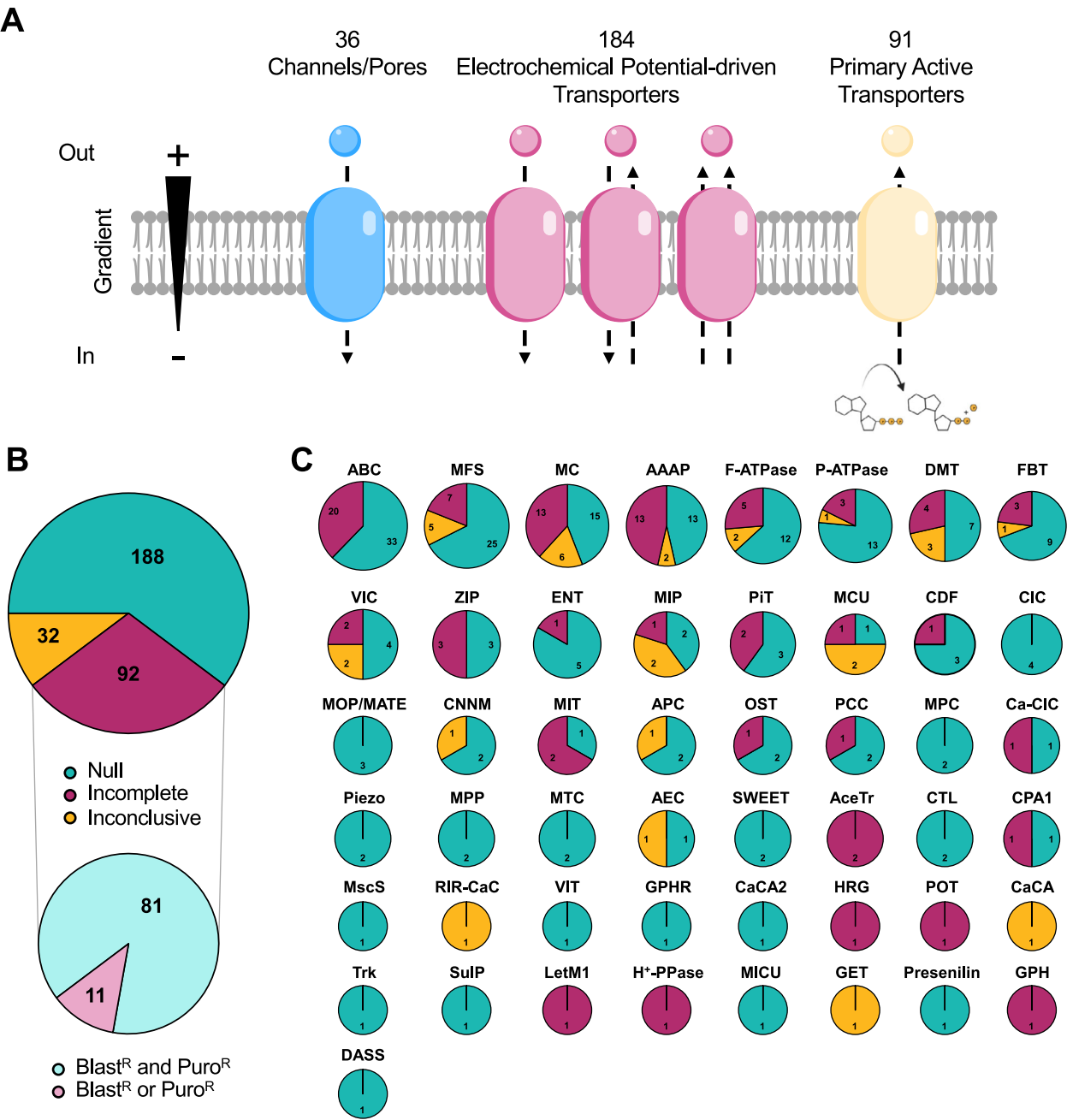
Fig. 2 | Generation of the TransLeish knockout library. A Overview of the number of predicted protein components of channels, carriers and pumps targeted for gene deletion in L. mexicana . B Summary of gene deletion results. The pie-charts show the numbers of successful deletions ('null'), incomplete deletions and inconclusive results. The category 'incomplete deletions' contained cell populations that were resistant to both selection drugs (Blasticidin and Puromycin) and
