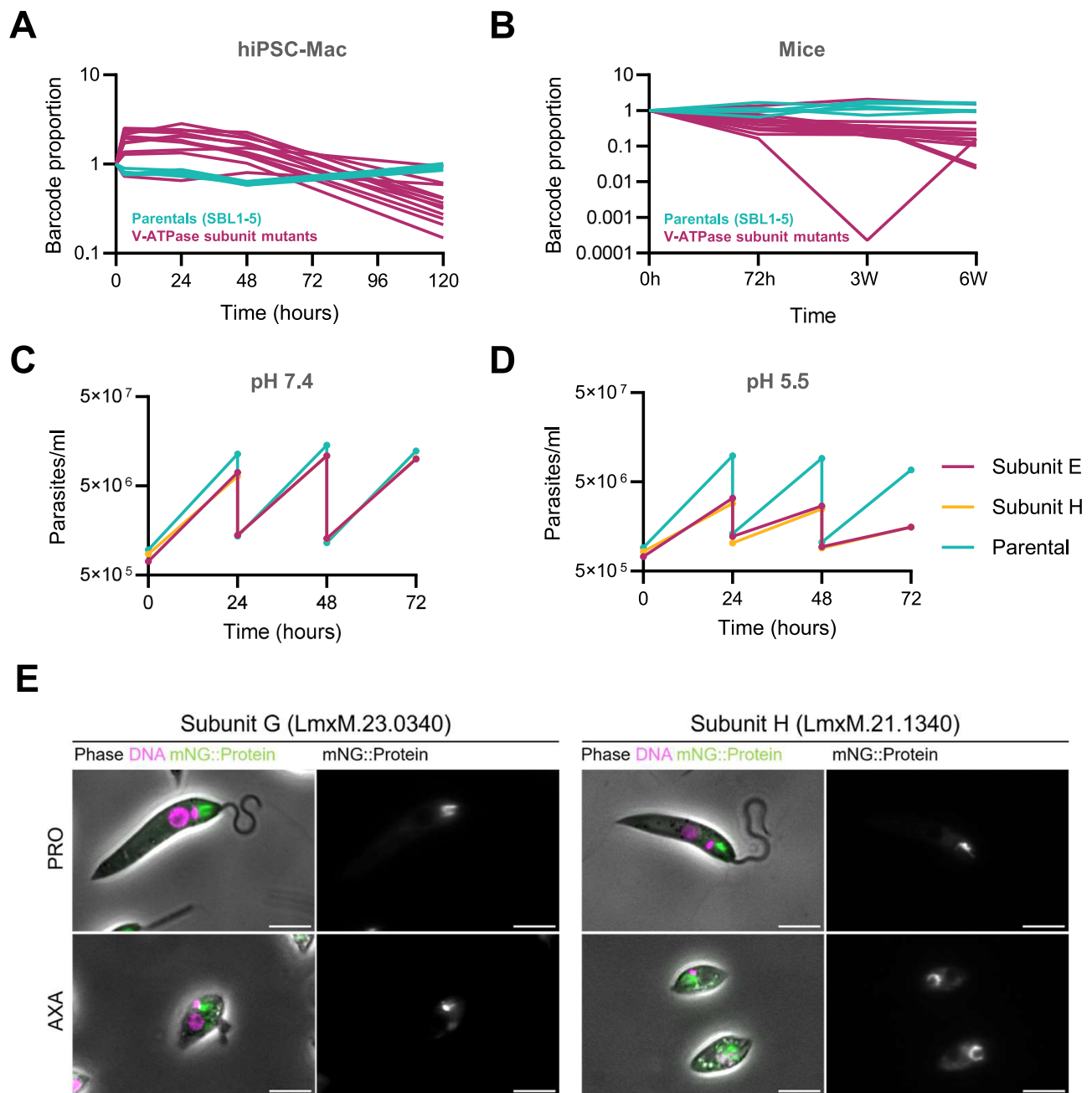
Fig. 7 | V-ATPase mutants show significant loss of fitness in macrophages and mice and reduced growth rates under low external pH conditions. A Barcode trajectories of barcoded parental controls and V-ATPase knockout mutants in macrophages. B Barcode trajectories in mice. C Growth of promastigote form V-ATPase deletion mutants V 1 E and V 1 H and the parental cell line in standard M199 medium at pH 7.4. Cells were diluted into fresh medium to a density of 1 \times 10^6 cells/ml every 24 h. Each point represents the average cell density measured from three separate cultures. D Growth profiles as in C, in M199 medium adjusted to pH 5.5. E Fluorescence micrographs showing the localisation of mNeonGreen-tagged V-
