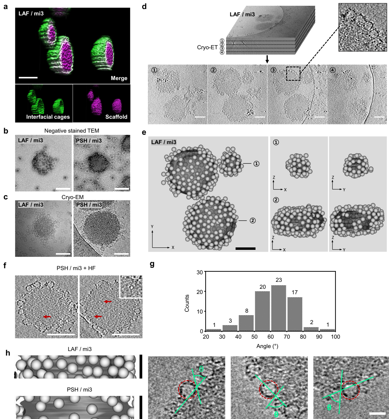
Fig. 4 | Structures of surface-stabilized protein condensates with interfacial protein cages. a Confocal Z-stack 3D representation of mi3-LAF condensates (LAF: magenta, mi3: green). b Negative-stained TEM images of mi3-LAF (left) and mi3-PSH (right) condensates. c Cryo-EM images of mi3-LAF (left) and mi3-PSH (right) condensates. d Reconstructed tomograms of mi3-LAF condensates. Four images of equal Z-distances (~40 nm) are shown below to demonstrate cage distributions at the bottom/middle/top of the condensate. Thick black dots are 10 nm gold nanoparticles used as a fiducial marker. e 3D volume models of mi3-LAF condensates
