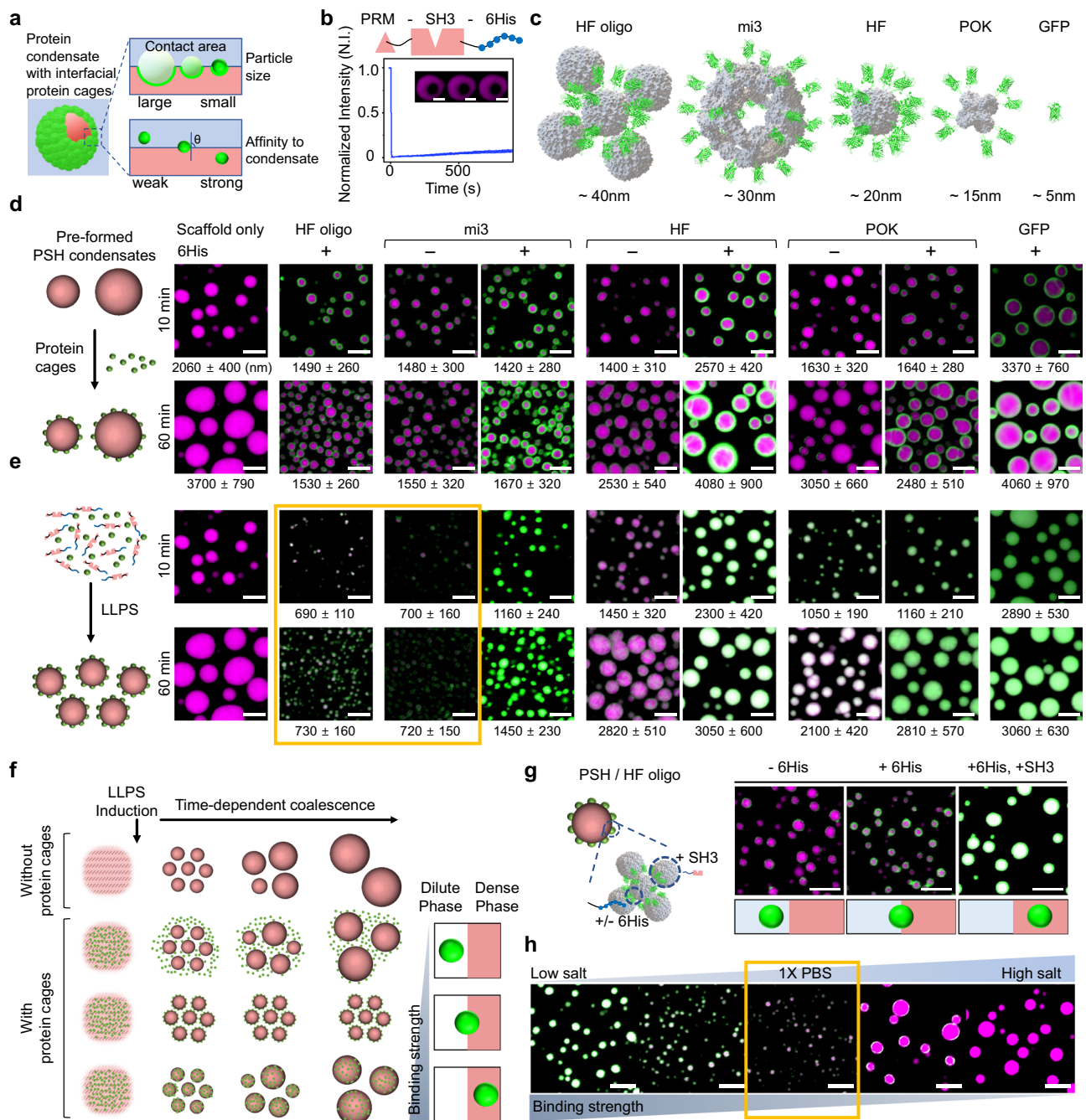
Fig. 1 | Assembly of surface-stabilized protein condensates with interfacial protein cages. a Schematic diagram of surface-stabilized (coalescence-inhibited) protein condensates with interfacial protein cages featuring optimized cage size and affinity to condensates. b FRAP recovery profile ( n = 10 condensates) and confocal images of bleached PSH (magenta) condensates. c Schematic structures of designed GFP (green)-fused interfacial protein cages. The approximate size of each cage is indicated below. d Sequential introduction (schematically expressed left) of HF oligo, mi3, HF, POK, and monomeric GFP with (+) or without (-) 6His to pre-formed PSH condensates. Confocal images of PSH condensates (magenta) without (scaffold only) or with added protein cages (green) after 10- and 60-min incubations are presented with average diameters shown below images. e Confocal
