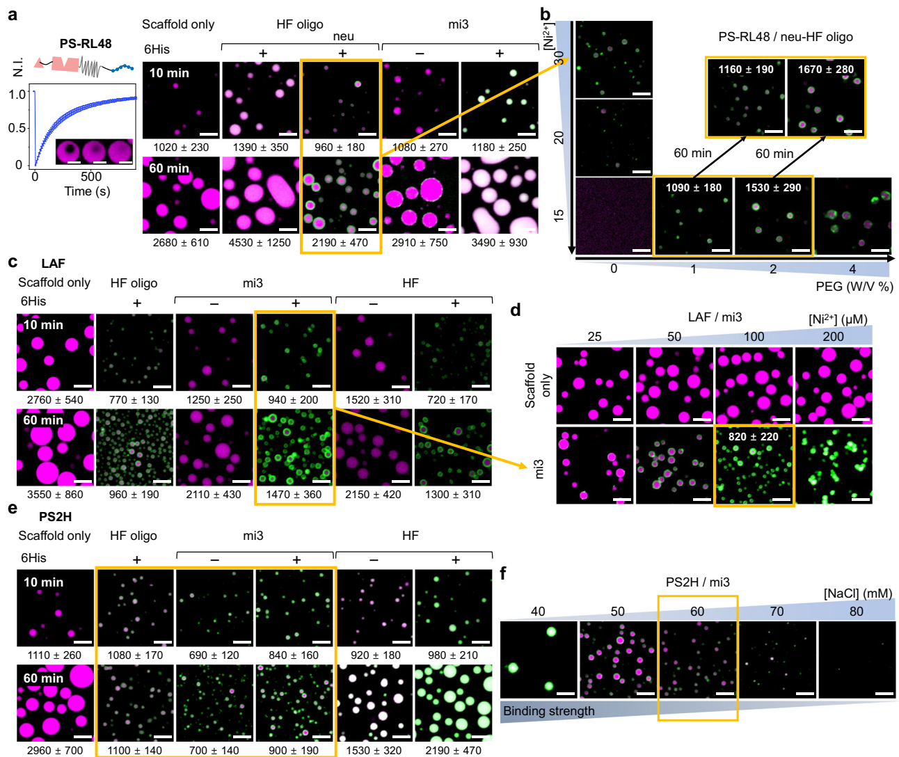
Fig. 2 | Surface stabilization for diverse fluidic protein condensates. a Confocal images of fluidic PS-RL48 condensates (FRAP data shown left, magenta, n = 10 condensates), phase separated in the presence of indicated protein cage variants (green) (one-pot assembly), after 10- and 60-min incubation with average diameters. Images for PS-RL48 condensates with neu-HF oligo that has undergone additional optimization (a yellow arrow) are marked with a yellow box. b Confocal images of neu-HF oligo-treated PS-RL48 condensates with systematically varied interaction strengths between neu-HF oligo and PS-RL48. [Ni^{2+}] was decreased to reduce interaction strength, and PEG was added to stimulate LLPS. Effectively stabilized (coalescence-inhibited for 60 min) condensates were indicated with yellow boxes with average diameters. c Confocal images of cage-treated (one-pot)
