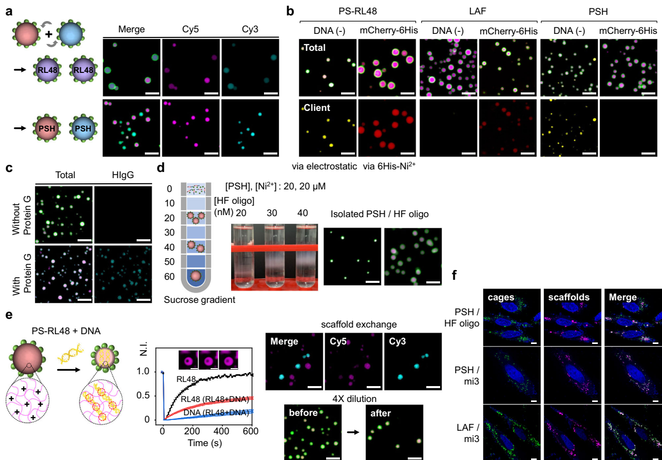
Fig. 5 | Dynamic behaviors of cage-stabilized protein condensates. a Confocal images of separately labeled (Cy5 magenta, Cy3 cyan) cage-stabilized condensate mixtures after 10 min incubation upon mixing (top: PS-RL48 condensates, bottom: PSH condensates). b Confocal images of cage-stabilized condensates with externally added client biomolecules (DNA (yellow) and mCherry-6His (red)). c Confocal images of HF oligo-PSH condensates (with or without protein G fusion to PSH) assembled with antibody (cyan). d Sucrose gradient centrifugation of cage-stabilized PSH condensates. A picture of sucrose gradient centrifuged HF oligo-PSH condensates with different sizes with schematics and exemplary confocal images of isolated PSH condensates in sucrose solution are shown. e Fluidity change of cage-stabilized condensates. DNA recruited into fluidic PS-RL48 condensates induces
