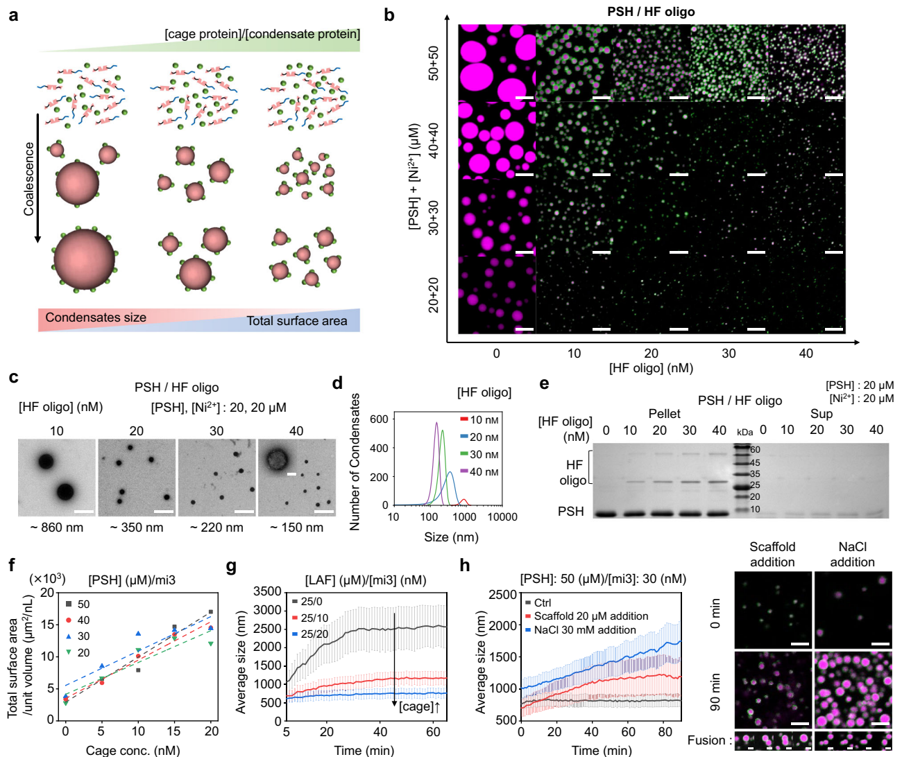
Fig. 3 | Size-controlled assembly of cage-stabilized protein condensates.
