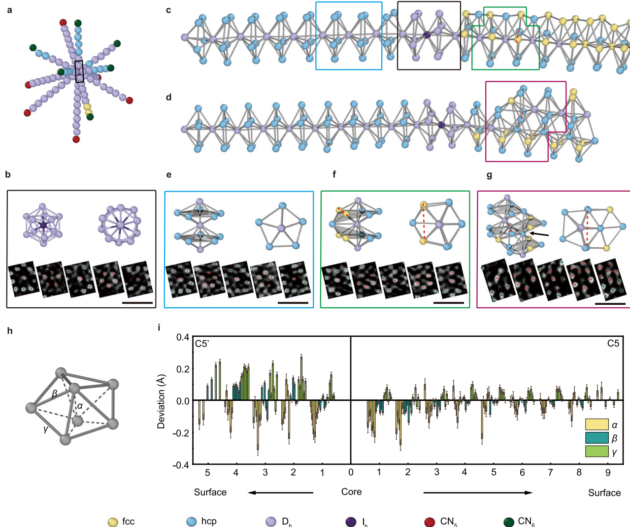
Fig. 2 | The two-sided coordination environment and bond length distribution in the fivefold axes. a Twelve axes of ICNP-1, consisting of six C5 and six C5' axes, with ending atoms marked as red and green, respectively. b Front and top views, and atomic slices through the raw reconstruction of the central icosahedron, enlarged from the black box in (a) . Scale bar: 1 nm. c , d Two types of atom columns composed of one C5 axis and one C5' axis. The edge dislocations change the coordination of axial atoms either to become 13-coordinated pseudo- D_h atoms ( c ), or to slip into the adjacent parallel column to form a new axis ( d ). e–g Front and top views, and atomic slices through the raw reconstruction of the repeating coordination units, enlarged from the blue, green and purple box in (c, d) , respectively. The gray shadows highlight the coordination planes above and below the center atom. Scale bar: 1 nm. h An ideal decahedron consisting of three types of atomic bonds. The \alpha , \beta , and \gamma represent the capping, capping-ring, and ring atom bonds, respectively. i The deviations of averaged bond lengths of \alpha (yellow), \beta (dark green), and \gamma (light green) from the outer surface of C5' axes to the outer surface of C5 axes, by subtracting the standard Au–Au bond length (2.88 Å). The distance between two neighboring D_h atoms, \alpha , is more and more compressed from C5 axes to C5' axes. \beta remains compressed in C5 axes but becomes stretched in C5' axes. The \gamma bonds are stretched in both C5 and C5' axes. The error of averaged bond length of \alpha , \beta , and \gamma bonds are estimated using the standard deviation of the bond length (Supplementary Note 2). The confidence interval in (i) is 95%. The balls in the atomic model with yellow, blue, light purple, and dark purple color represent the atoms with fcc, hcp, D_h , and I_h structure, respectively. The balls in the atomic model with red and green color represent the ending atoms in fivefold and sixfold axis, respectively. Source data are provided as a Source Data file.
