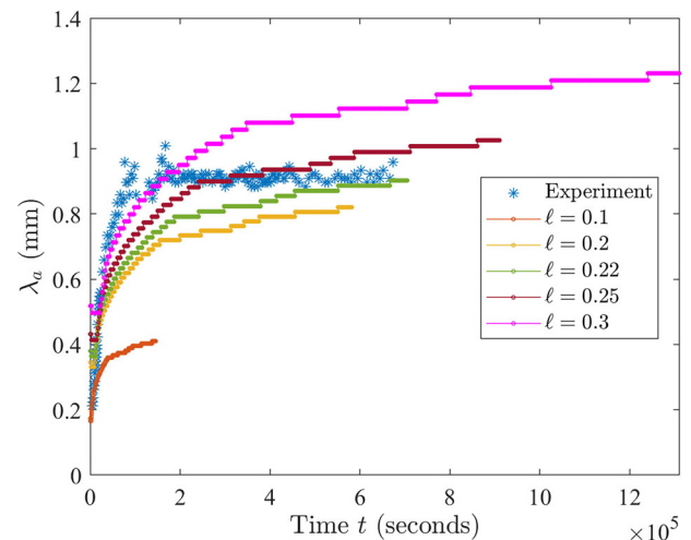
Fig. 13 | Dominant length scale \lambda_a vs. t for BCAT-5 Sample 7, obtained from numerical simulations using \gamma = 130 , plotted with the experimental data (blue points). The different colors correspond to different choices of \ell (in mm) used in computing the length and time scales L and \tau defined in Eq. (10).
