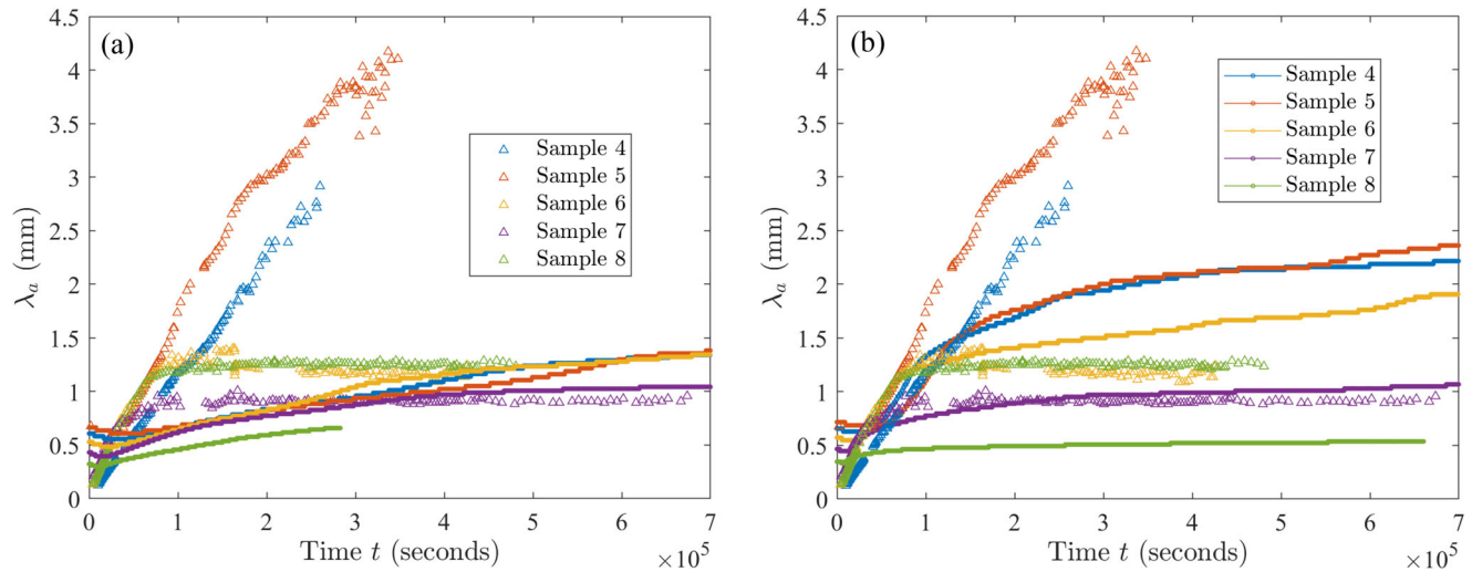
Fig. 14 | Comparison between experiment and theory. Dominant length scale \lambda_a(t) in BCAT-5 Samples 4, 5, 6, 7 and 8, obtained from experimental data (triangles) and simulations (solid curves) run without accounting for hydrodynamic interactions
