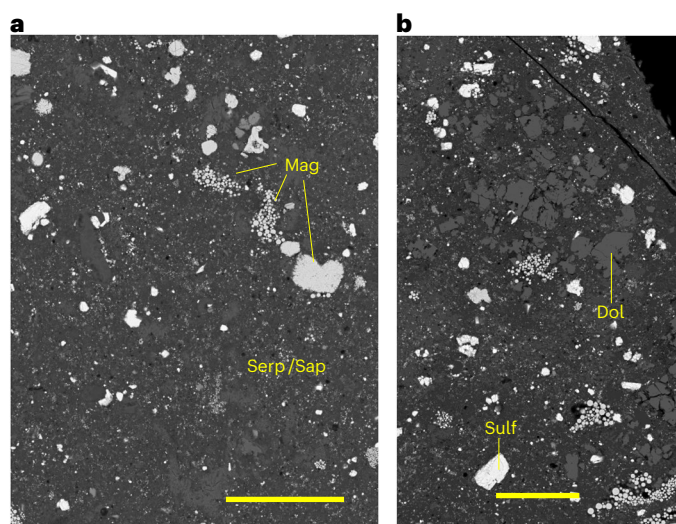
Fig. 1 | Backscattered images from two areas of particle C0068 illustrating the heterogeneous nature of the Ryugu material 7 . a , Magnetite (Mag) occurs both as clusters of framboids and spherical aggregates. The dominant, fine-grained dark material comprises intergrown serpentine and saponite (Serp/Sap). The fine-grained dark matrix represents intergrown serpentine and saponite. b , A large number of relatively coarse-grained dolomite crystals (Dol) are present along the right-hand edge. Sulfide crystals (Sulf) of varying grain sizes can also be seen. Scale bars, 25 \mu\text{m} .
