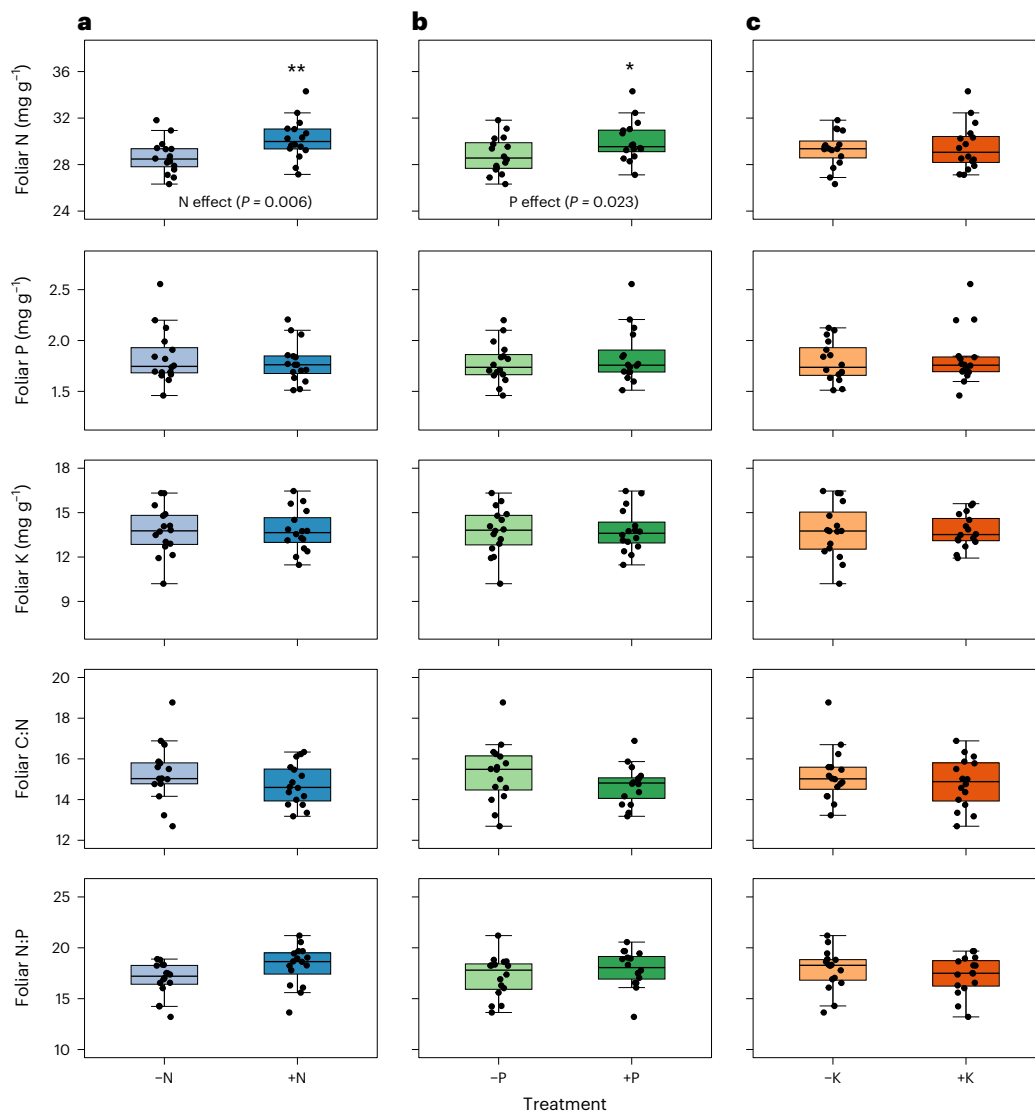
Fig. 3 | Nutrient addition effects on sunlit foliar chemistry, weighted by the importance value index of the sampled five dominant tree species in each replicate plot, at the nutrient addition experiment in Budongo Forest Reserve, Uganda. a–c , Box plots (25th quartile, median and 75th quartile) and whiskers ( 1.5 \times interquartile range) of foliar chemistry ( n = 16 plots) in treatments with or
