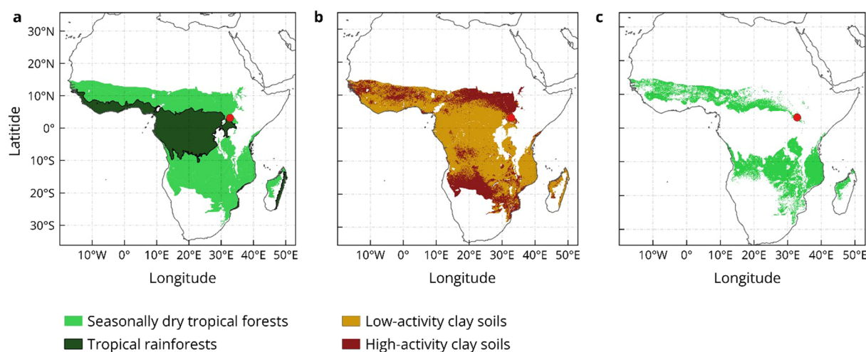
Extended Data Fig. 2 | Extent of seasonally dry Afrotropical forests on heavily weathered soils, showing study location in Uganda (red dot).
