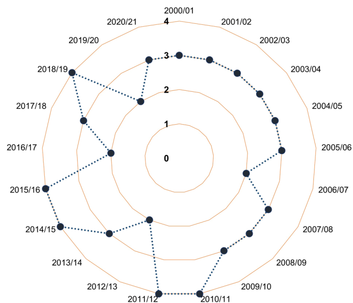
Extended Data Fig. 1 | Dry season lengths (number of months with precipitation < 100 mm month -1 ) at the Budongo Forest Reserve, Uganda. Data extends from 2000 to 2021 measured at the Budongo Conservation Field Station. Nutrient addition experimental period was from 2018 to 2021; the
