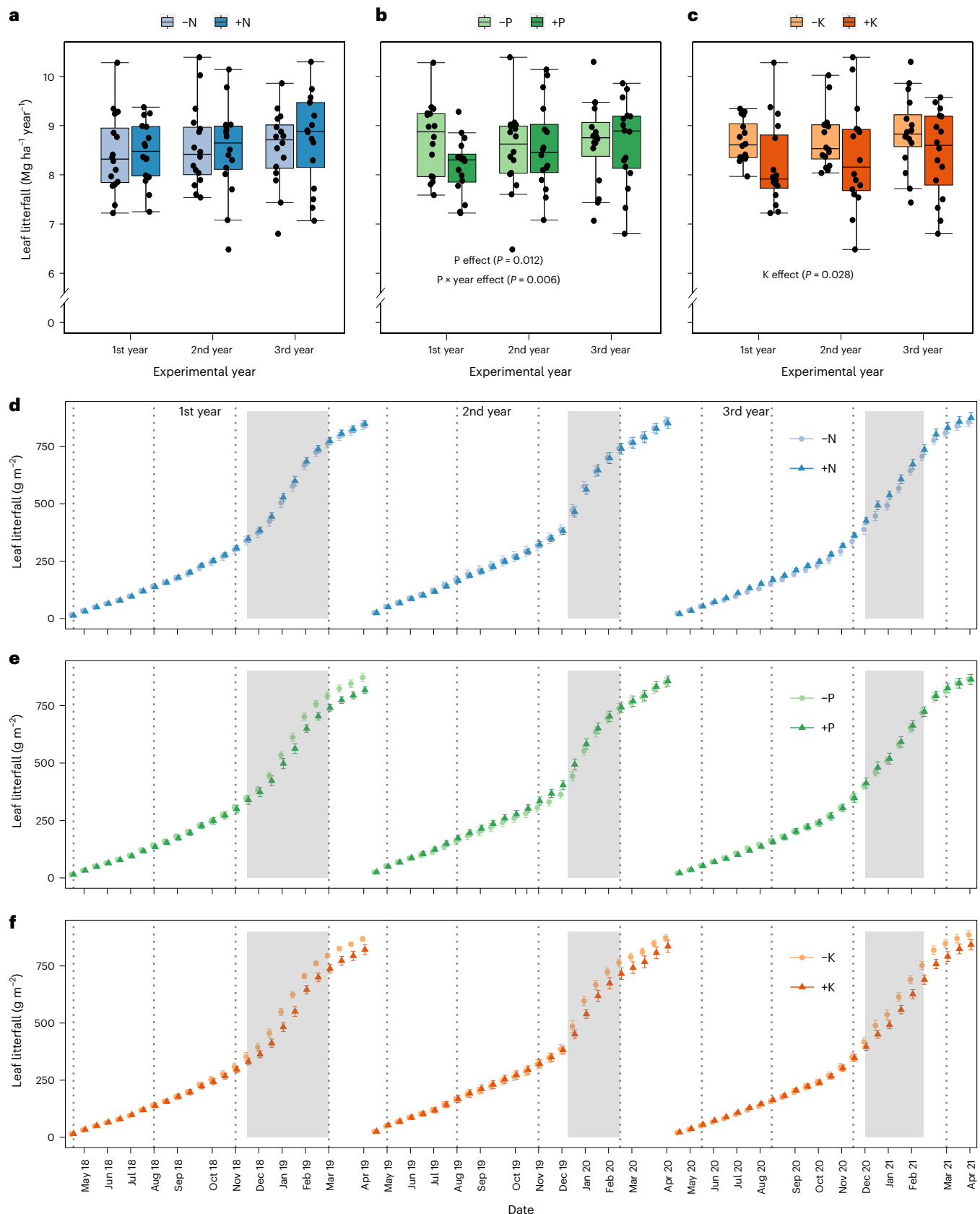
Fig. 1 | Nutrient addition effects on leaf litterfall in Budongo Forest Reserve, Uganda. a–f , Box plots (25th quartile, median and 75th quartile) and whiskers ( 1.5 \times interquartile range) of annual leaf litter production ( a–c ; n = 16 plots) and cumulative leaf litterfall ( d–f , mean \pm standard error of the mean (SEM); n = 16 plots) measured bi-weekly from May 2018 to April 2021, pooled for plots with or without nitrogen (+N vs -N; a,d ), phosphorus (+P vs -P; b,e ) and potassium (+K vs -K; c,f ). b–c and e–f show the reduction effects of P addition in the first year and
