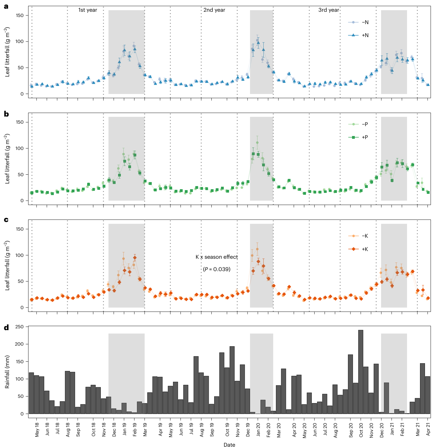
Fig. 2 | Temporal response of leaf litterfall to nutrient additions in Budongo Forest Reserve, Uganda. a–c, Bi-weekly leaf litter production (mean \pm SEM, n = 16 plots) measured from May 2018 to April 2021, pooled for plots with or without nitrogen (+N vs –N; a ), phosphorus (+P vs –P; b ) and potassium (+K vs –K; c ). c, The four-week delayed peak of leaf litterfall in +K treatments during the first
