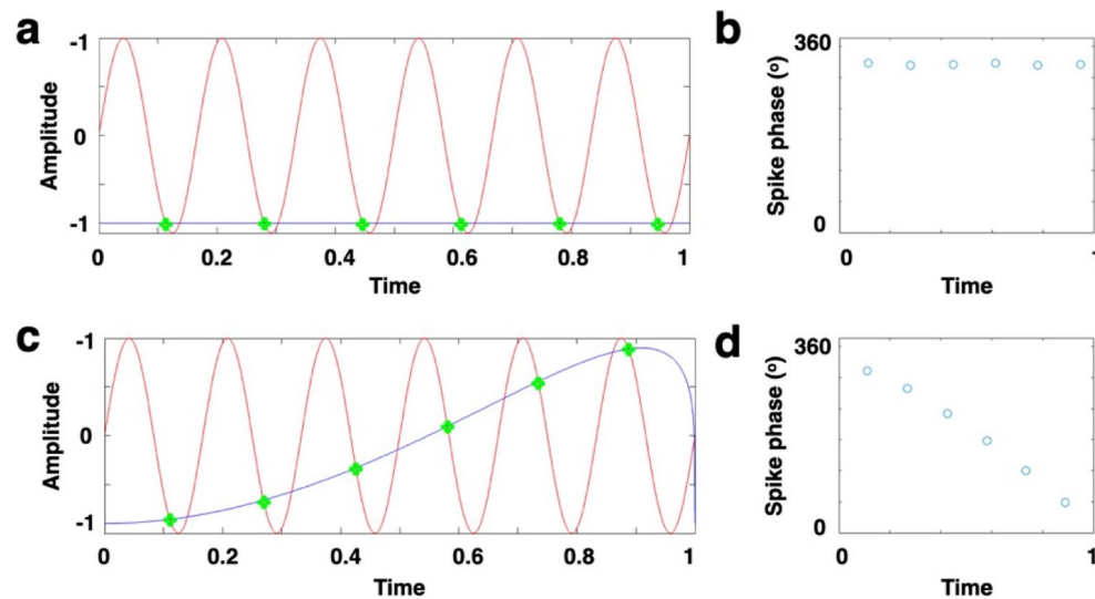
Extended Data Fig. 9 | Phase precession can exist without firing rate modulation. Simulation based on the model of Mehta et al, 2002. ( a and c ) The spikes in this model (green dots) occur when the down-swing of the fluctuating inhibitory current (red) crosses the excitatory current (blue). Like in the original implementation, in this simulation neurons fired only briefly when excitation
