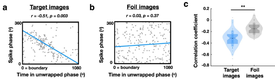
Extended Data Fig. 8 | Comparison of phase precession when recognizing target (old) versus foil (new) images. An example MTL neuron showing phase precession when the participant is asked to recognize target images ( a ) and foil images ( b ). Note that no significant phase precession is observed when identifying foil images. ( c ) Comparison between phase precession strength (correlation coefficient values) when participants are instructed to recognize target (blue) versus foil images (gray) across all phase precession neurons identified during scene recognition ( n = 51 ). Each dot represents one neuron.
