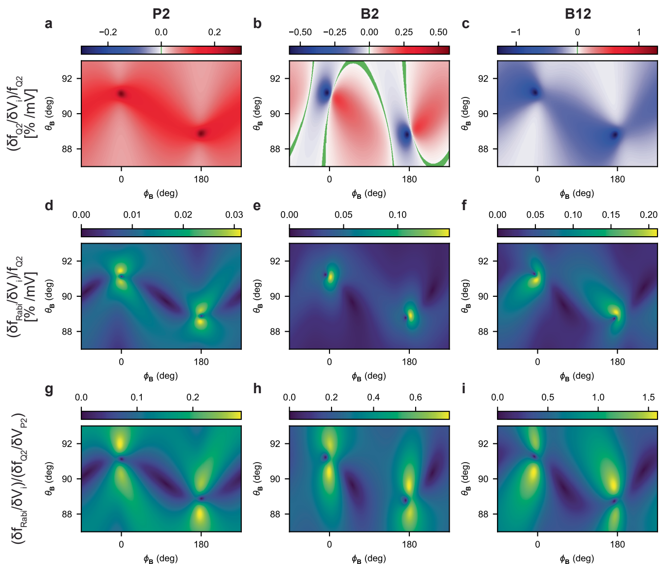
Extended Data Fig. 4 | Longitudinal and transverse components of the fitted \partial \bar{g}/\partial V_i . a–c. Using the fitted \partial \bar{g}/\partial V_i , as detailed in Fig. 4 of the main text and Extended Data Table 1, we plot the expected normalized resonance frequency fluctuation of Q2 as a result of a voltage fluctuation on gate P2 ( a ), B2 ( b ), and B12 ( c ) for different magnetic field orientations. Zero crossings are marked in green, to indicate the presence of a true sweet spot. d–f. Expected normalized Rabi
