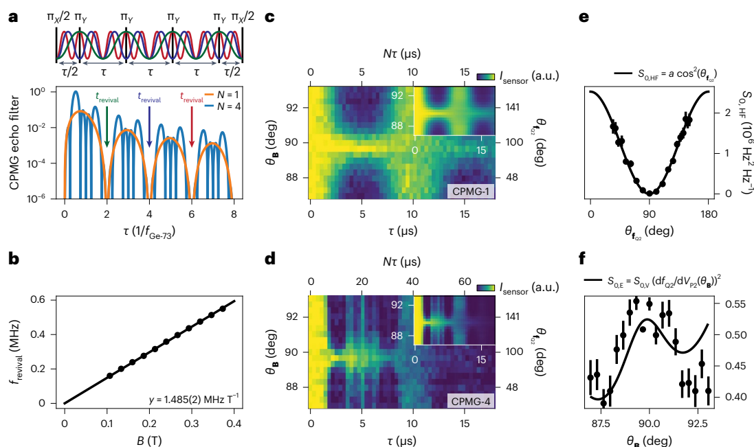
Fig. 5 | Collapse and revival of qubit coherence due to hyperfine interaction.
