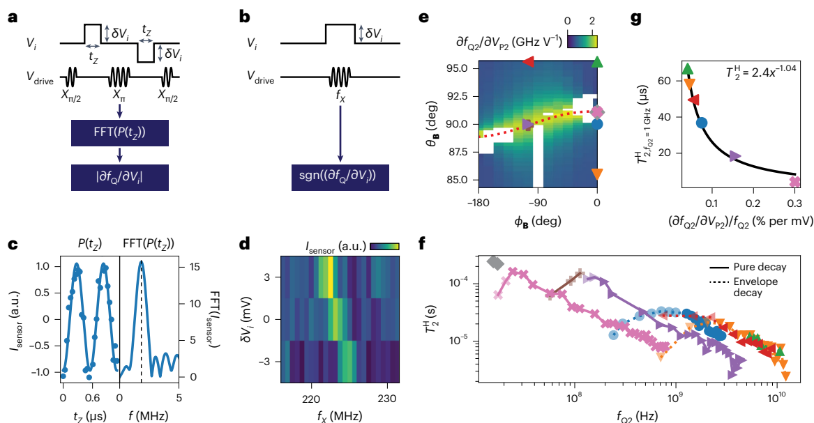
Fig. 3 | Electric field sensitivity and coherence dependence on magnetic field orientation. a , Pulse sequences used to measure the voltage sensitivity of the energy splitting \partial f_Q/\partial V_i . A positive (negative) voltage pulse \delta V_i of varying length t_z is applied to the test gate electrode i in the first (second) free evolution of a Hahn echo to extract |\partial f_Q/\partial V_i| . b , Pulse sequences used to infer the sign of \partial f_Q/\partial V_i by assessing the shift in the qubit resonance frequency as a result of a voltage pulse \delta V_i . c , Left: spin-up probability P(t_z) as reflected by the charge sensor current I_{\text{sensor}} as a function of the pulse length t_z , where the solid line is a fit to the data points. Right: fast Fourier transform (FFT) of I_{\text{sensor}} , enabling the extraction of |\partial f_Q/\partial V_i| . d , I_{\text{sensor}} as a function of the drive frequency f_x and \delta V_i . The shift in the resonance frequency enables the sign of \partial f_Q/\partial V_i to be extracted. e , The qubit energy splitting sensitivity to a voltage change on the plunger gate \partial f_{Q2}/\partial V_{P2} , as a function of different magnetic field orientations \phi_B and \theta_B . B is adapted to keep f_{Q2} constant at f_{Q2} = 1.36(7) GHz. Data acquisition is hindered for the white areas as
