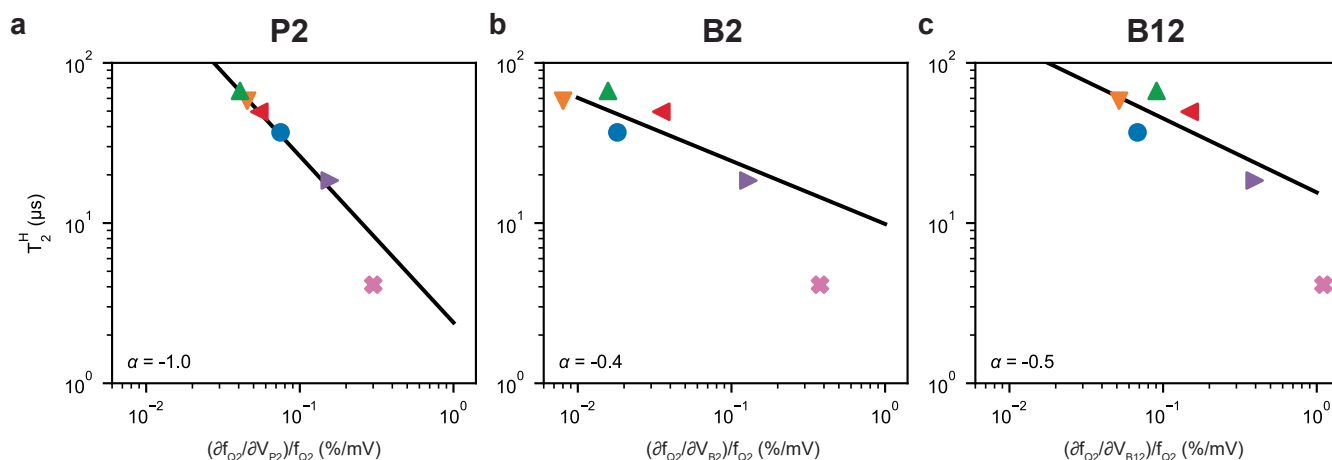
Extended Data Fig. 3 | Q2 coherence as a function of the different gate voltage sensitivities. a–c , Observed Hahn echo coherence time (data from Fig. 3g in the main text), as a function of the relative qubit frequency sensitivity (\partial f_{Q2}/\partial V_i)/f_{Q2} to a voltage fluctuation on gate P2 ( a ), B2 ( b ), or B12 ( c ). Voltage sensitivities are obtained from the data for gate P2 (Fig. 3e) from the fits of \delta\vec{g} presented in Fig. 4 of the main text, as well as Extended Data Fig. 4 for gates B2 and B12. Black lines are fits to a power law T_2^H = a \exp(((\partial f_{Q2}/\partial V_i)/f_{Q2})^\alpha) , with a a scaling factor and \alpha
