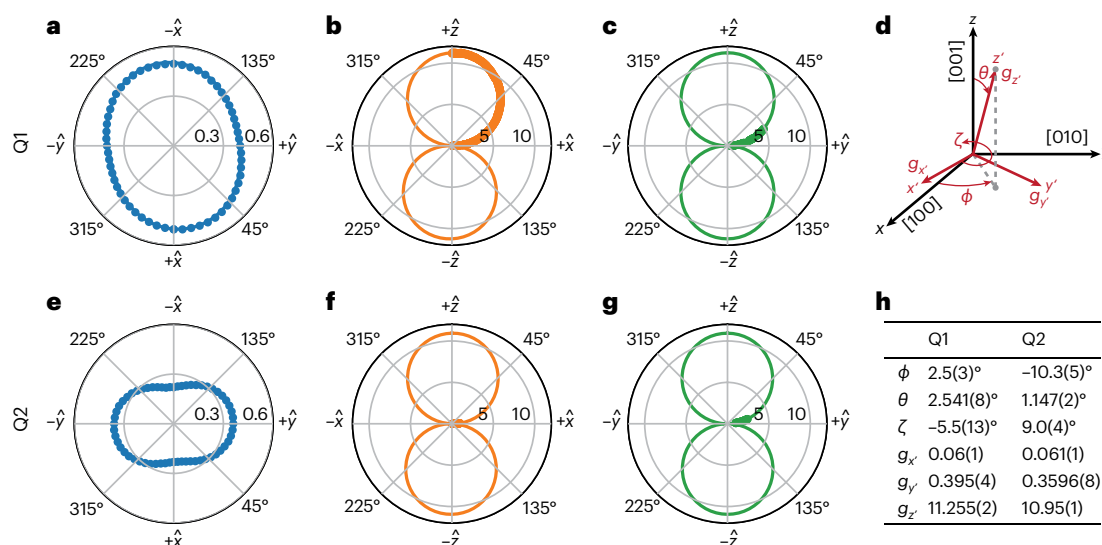
Fig. 2 | Measurement of the hole \vec{g} -tensor. a–c, e–g. Cross-section of \vec{g} of Q1 (a–c) and Q2 (e–g) in the x – y plane (a, e), x – z plane (b, f) and y – z plane (c, g) of the magnet frame. Dots indicate measurements of \vec{g}^* and the solid line corresponds to the fit of \vec{g} . Exemplary resonance spectra used to extract \vec{g} are plotted in Supplementary
