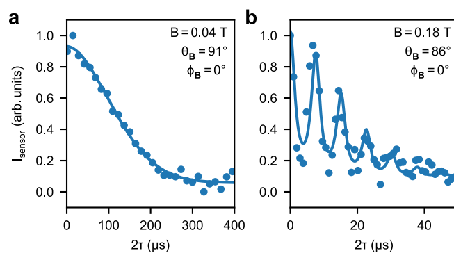
Extended Data Fig. 2 | Hahn echo decay of Q2. a , Hahn echo decay of Q2, for the magnetic field aligned with the hyperfine sweet plane. Solid line is a fit to the data used to extract T_2^{\text{H}} . b , Hahn echo decay of Q2, for the magnetic field aligned away
