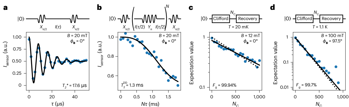
Fig. 6 | Coherence figures at low magnetic field in the hyperfine sweet spot.
