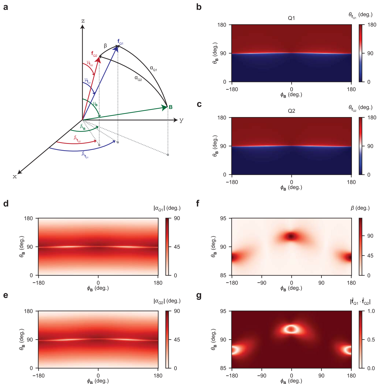
Extended Data Fig. 1 | Projections of the fitted g -tensors. From the experimentally extracted the qubit g -tensors, we calculate the qubit quantisation axis hf_Q = \mu_B \vec{g} \mathbf{B} as a function of \mathbf{B} . a , Diagram illustrating the relevant angles. \theta_B and \phi_B are the elevation and azimuth angle of the applied magnetic field respectively. \theta_{Q_i} and \phi_{Q_i} are the elevation and azimuth angle of the resulting Larmor vector of Q_i . \alpha_{Q_i} is the angle between the applied magnetic field and the resulting Larmor vector of Q_i and \beta is the angle between the two quantisation axes of the two qubits. b, c , Elevation angle of the Larmor vector of Q1 ( b ) and Q2 ( c ), as a function of the orientation of the magnetic field. As a result of the large anisotropy of \vec{g} , the quantisation axis of the qubit rapidly flips from \mathbf{f}_{Q_i} \parallel \mathbf{z} to
