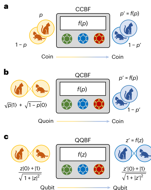
Fig. 1 | Conceptual scheme of a Bernoulli factory. a , CCBF where a sequence of classical coins with unknown bias p are processed for producing a new coin with bias f(p) (refs. 22,44). b , QCBF in which a quoin serves as the input to synthesize a classical one 25,26 . c , Fully quantum version where both input and output are general quantum states 29 .
