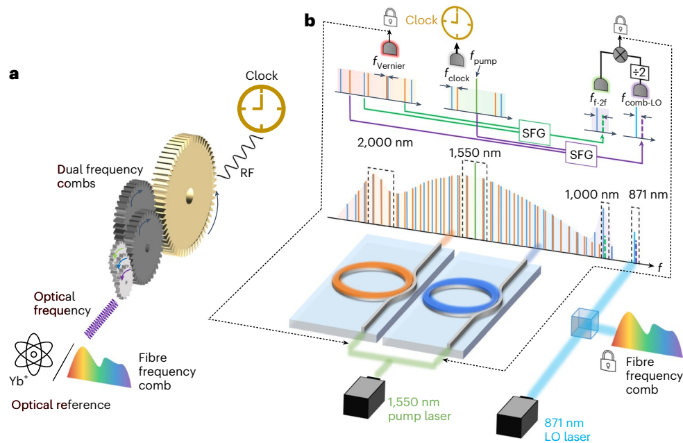
Fig. 1 | Overview of Vernier dual-microcomb scheme for OFD. a , An optical frequency comb system is analogous to a gear set, transferring the stability from optical frequency to RF. The large (small) size gears represent radio (optical) frequencies. The Vernier dual comb can further downconvert the RF by beating against each other. The optical reference can be a Yb + ion trap (as our system is designed for) or a stabilized FC (as a stable frequency proxy we adopted). b , An illustration of a Vernier dual-microcomb system for OFD. The dual combs excited by a shared pump at 1,550 nm generate broadband spectra spanning from ~1 \mu m
