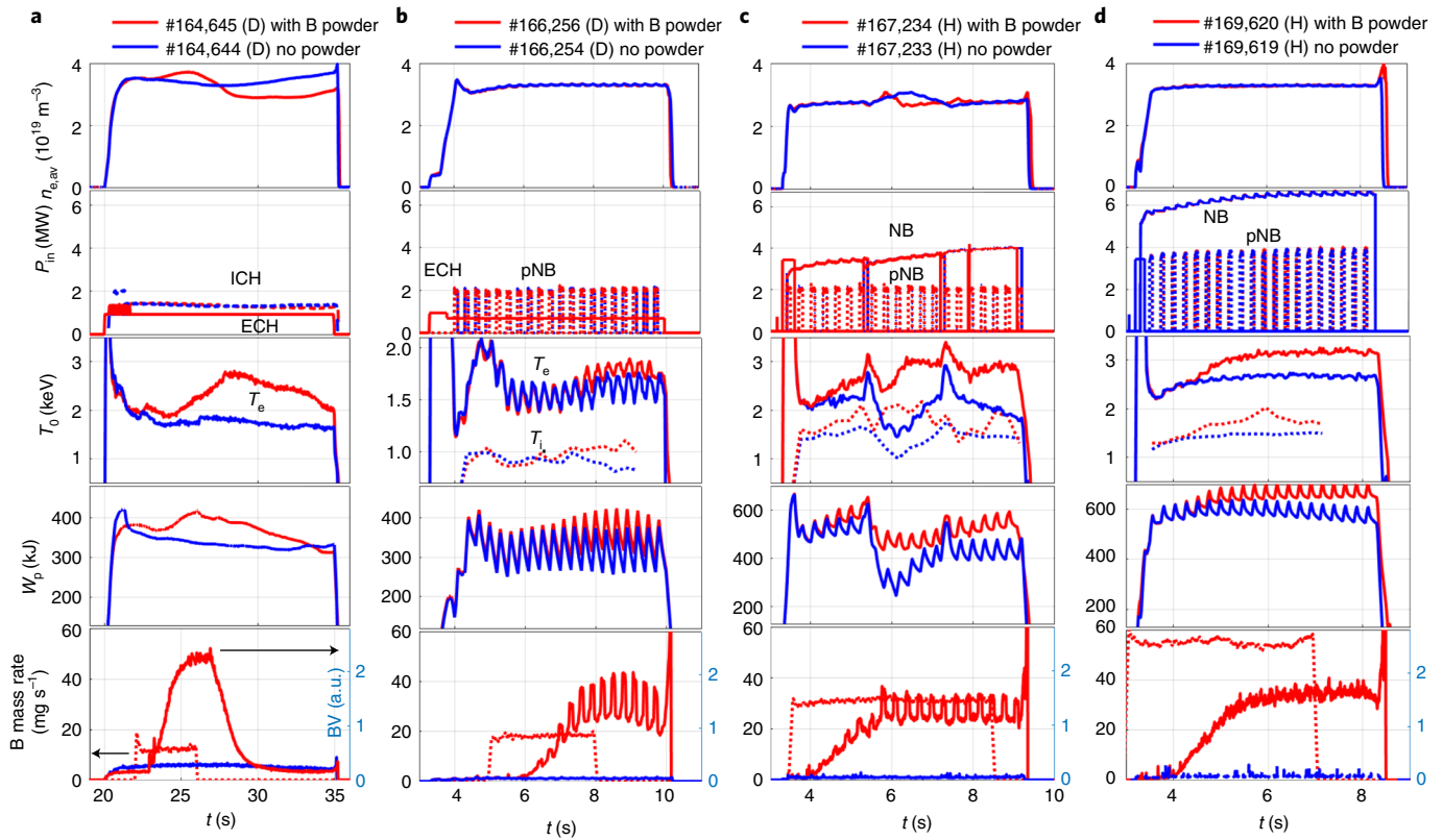
Fig. 1 | Time traces of discharges with improved performances during boron powder injection. a–d, From top to bottom: line-averaged density n_{e,av} ; input power P_{in} separated by different sources: ion and electron cyclotron resonant heating (ICH, ECH), tangential neutral beam (NB) and perpendicular diagnostic beam (pNB); electron (solid) and ion (dotted) temperature T_e and T_i ; stored energy W_p ; injected boron mass rate (dotted, left axis) and BV spectroscopic line (solid, right axis). Red colour for shots with B powder injection, blue for reference shots (no powder). Main plasma ion is D for a and b and H for c and d . The magnetic field direction for d is reversed with respect to a–c .
