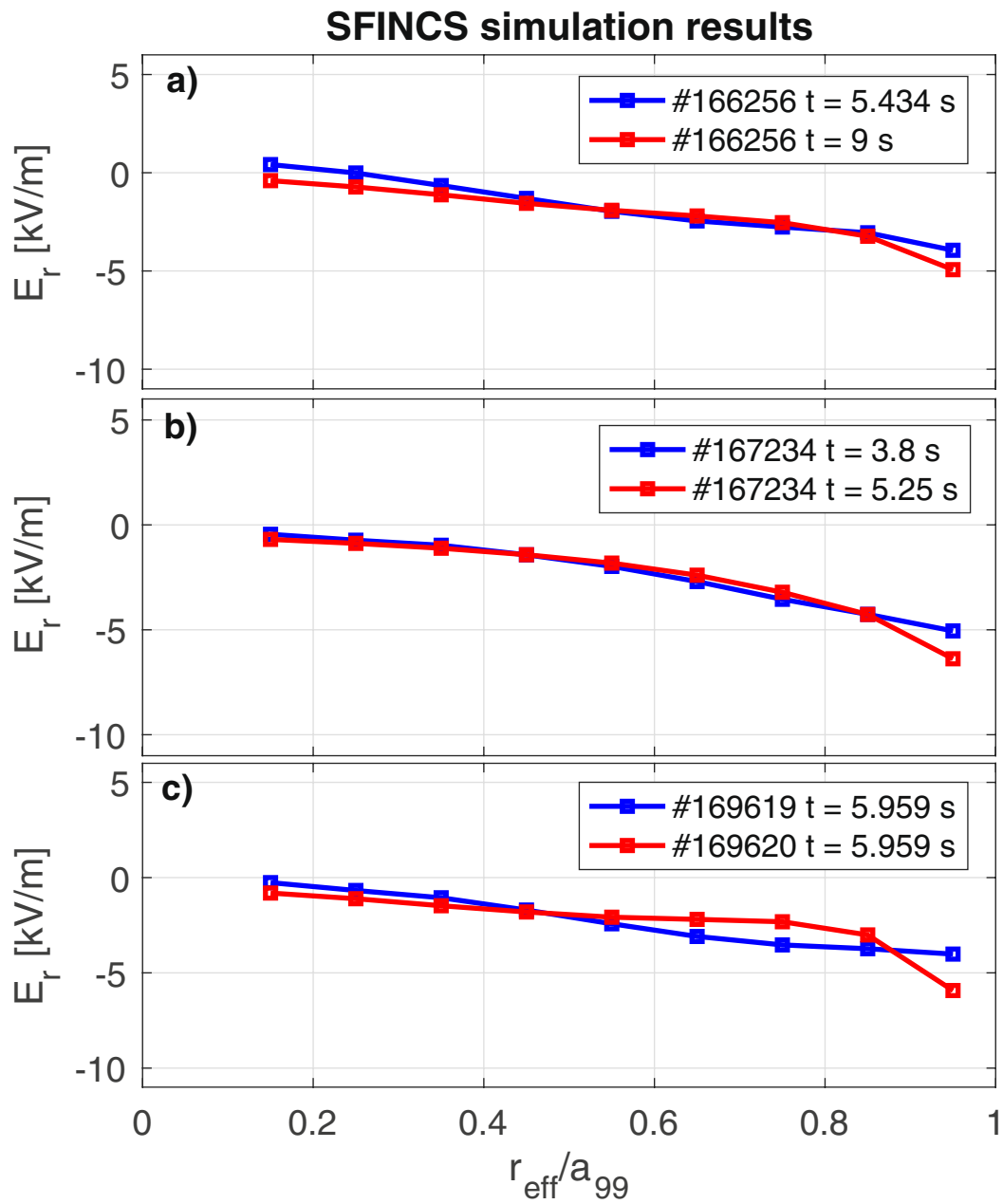
Extended Data Fig. 1 | Ambipolar radial electric field E_r resulting from neoclassical simulations. E_r resulting from SFINCS simulations are plotted as a function of the normalized effective minor radius r_{\text{eff}}/a_{99} for the cases in Fig. 1b–d (no T_i measurement is available for case in Fig. 1a). For each subplot, E_r during boron powder injection (red) is compared with its reference case without powder injection (blue). For a) and b), the reference case is the same discharge at a time before powder injection. For case c) the reference case is an identical discharge without powder injection, at the same time.
