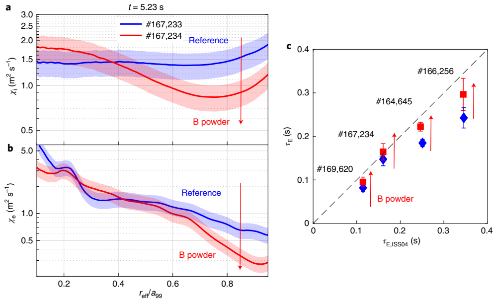
Fig. 6 | Energy transport reduction and confinement improvement. a, b, Radial profiles of heat conductivities for ions \chi_i ( a ) and electrons \chi_e ( b ) as a function of the normalized effective minor radius r_{\text{eff}}/a_{99} , comparing a discharge with powder injection (red) with a reference discharge (blue). Shaded areas represent an estimated average relative error of 20% on the DYTRANS analysis results, obtained by comparing different time frames of the simulation. c, Measured energy confinement time \tau_E during B powder injection (red squares) and for the reference shots at the same time (blue diamonds). The experimental \tau_E is plotted against the predicted energy confinement time from the international stellarator scaling T_{E,\text{ISS04}} (ref. 26 ). Error bars represent standard deviation in time over a window of 200 ms.
