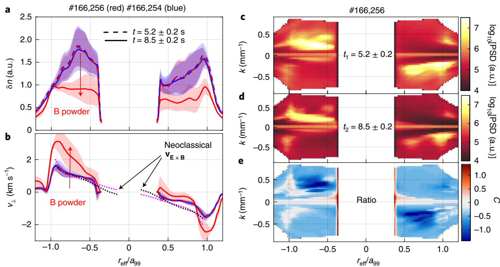
Fig. 4 | Suppression of turbulent fluctuations. a,b , Radial profiles of turbulent fluctuation amplitude \delta n ( a ) and the perpendicular velocity v_{\perp} ( b ) for a powder injection shot (#166,256, red) and its reference (#166,254, blue), at t = 5.2 s (before injection, dashed lines) and t = 8.5 s (during injection, solid lines). The radial profiles are averaged over a time window of 0.4 s to avoid instantaneous variations caused by the pulsed diagnostic neutral beam. The shaded area accounts for the standard deviation in time. In b , neoclassical estimates of \mathbf{E} \times \mathbf{B} velocity for #166,256 before (black) and during (magenta) powder injection are shown with dotted lines. c-e , Radially resolved PSD in terms of wave number for #166,256 before ( c ) and during ( d ) powder injection and their ratio ( e ) C as defined in equation (1).
