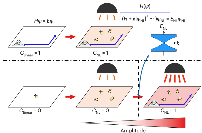
Fig. 1 | Schematic of the nonlinear Chern insulators and the nonlinearity-induced topological phase transition. Although the topology of a non-interacting linear system can be characterized by the Chern number that is computed from its eigenvectors, the topology of a nonlinear system is classified by the nonlinear Chern number, which utilizes the nonlinear extension of the eigenequation. In weakly nonlinear regions (that is, small amplitude), the nonlinear Chern number predicts the existence of edge modes corresponding to those in linear systems. Specifically, when nonlinear systems exhibit edge-localized steady states, both nonlinear and linear Chern numbers are non-zero (top). If we inject higher energy into the system and consider the eigenmodes with large amplitudes, the nonlinear band structure can become gapless. At such a gapless point, a nonlinearity-induced topological phase transition can occur, where topological boundary modes appear with the non-zero nonlinear Chern number (bottom). The nonlinearity-induced topological phases exhibit boundary modes that cannot be predicted from the linear Chern number. Therefore, such topological phases are genuinely unique to nonlinear systems.
