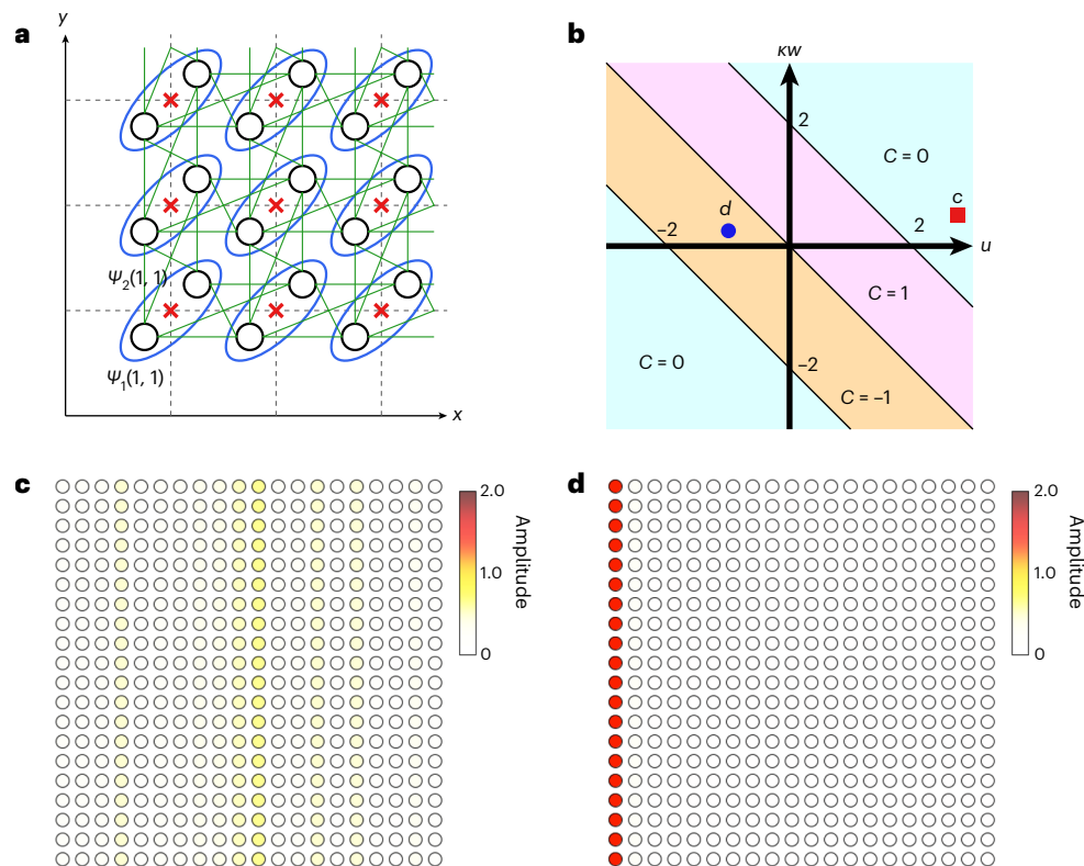
Fig. 2 | Phase diagram and dynamics of the nonlinear QWZ model.
