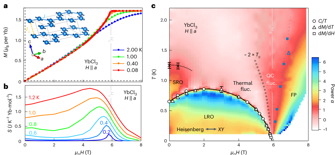
Fig. 1 | Magnetic-field-induced quantum phase transition and H - T phase diagram for \text{YbCl}_3 . a , The magnetization M(H) curves at different temperatures. The Van Vleck contribution has been subtracted (Supplementary Fig. 1). The inset shows the honeycomb layered structure of \text{YbCl}_3 (space group C12/m1 ) 26,41 with an antiferromagnetic intralayer coupling J \approx 5 K and a ferromagnetic interlayer coupling J_{\perp} \approx 0.1 mK. b , The magnetic field dependence of entropy at different temperatures. c , The H - T phase diagram. The power \alpha of the T -dependent specific heat C ( C \propto T^{\alpha} defined as \alpha(T) \equiv d \ln C / d \ln T ) was evaluated by linear fits to \ln C versus \ln T for every four data points and is indicated by the colour. The open symbols indicate the T_c of the long-range magnetic ordering, defined by the
