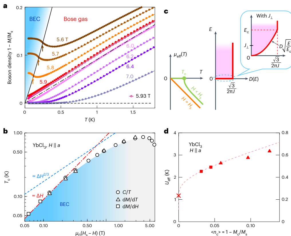
Fig. 3 | Quantum critical behaviour of magnetization M(T) and T_c(H) , and quasi-2D Bose gas model. a , Temperature dependence of boson density \langle n \rangle = 1 - M/M_s for various magnetic fields H around the QCP. The dashed line represents \langle n \rangle = T/T_0 , and T_0 = 11 \text{ K} = 2.2J . The arrows indicate T_c determined from the peak in dM/dT (Fig. 2e,f). The solid line represents \langle n_c \rangle = Dk_B T_{\text{BEC}} (-\ln(k_B T_{\text{BEC}}/E_c) + 2) with a cut-off energy E_c = 0.2 \text{ mK} and D = \sqrt{3}/2\pi J for J = 5 \text{ K} (Fig. 3c). b , Full logarithmic plot of T_c as a function of H_s - H , with H_s = 5.93 \text{ T} . The dashed and the broken lines represent T_c \propto (H_s - H) and (H_s - H)^{2/3} expected for 2D and 3D, respectively. c , The dilute Bose gas model used to analyse C(T) and M(T) around the QCP. The density of states D(E) for the 2D honeycomb tight-binding model has a bandwidth of 3J and a finite value at E = 0 , D = \sqrt{3}/2\pi J . In the presence of a small interlayer coupling J_\perp ( \ll J ), a 3D density of states with D(E) proportional
