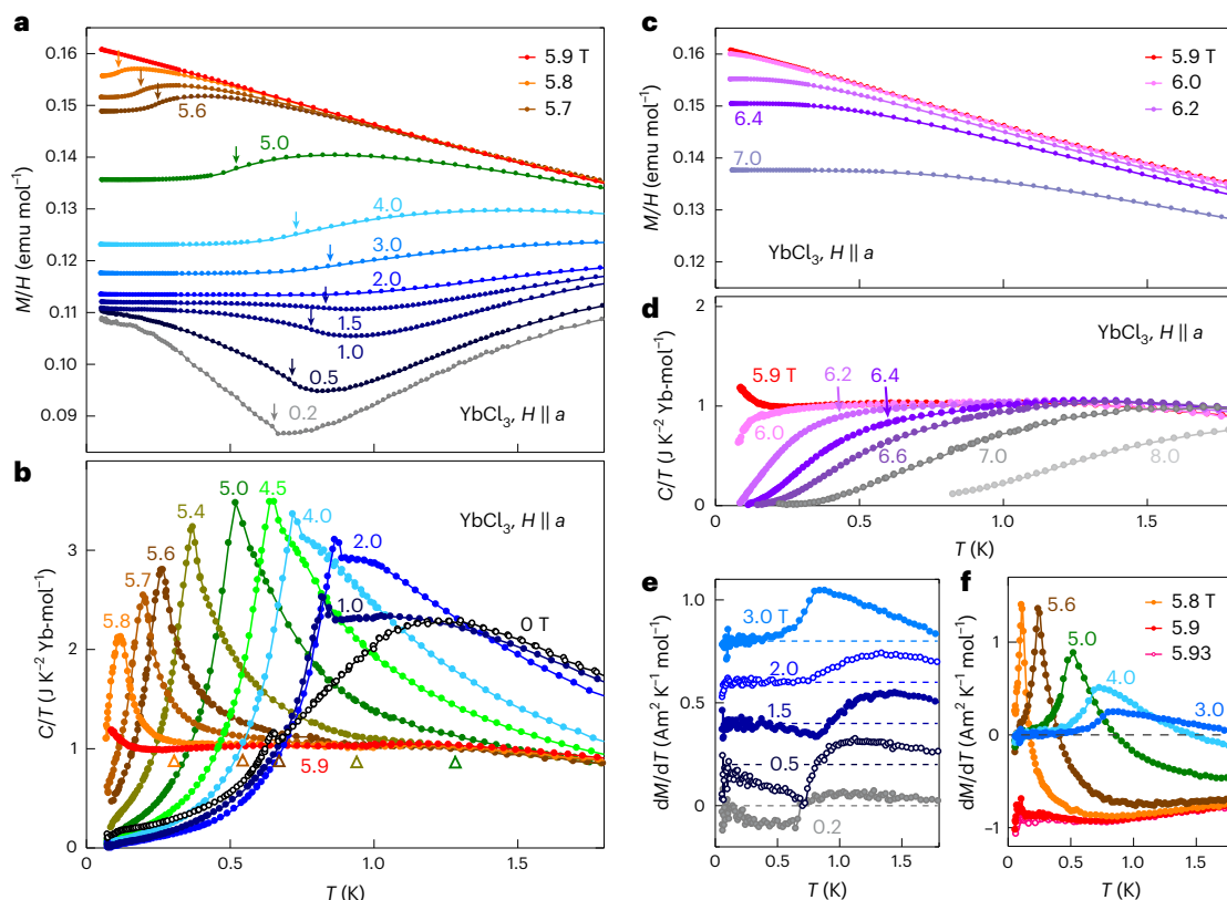
Fig. 2 | Temperature dependence of magnetization M(T) and specific heat C(T) at different magnetic fields. a, c, T -dependent M/H for H \leq H_s (a) and H \geq H_s (c). The arrows in a represent T_c determined from the singularity in dM/dT (e, f). b, d, T -dependent C/T for H \leq H_s (b) and H \geq H_s (d). Open triangles in b mark the
