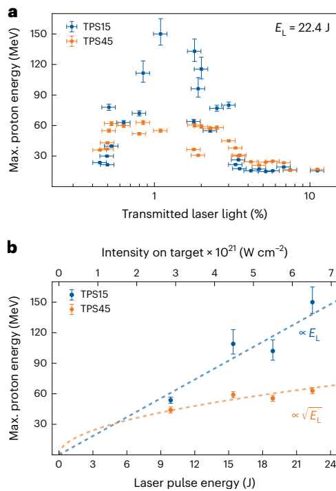
Fig. 2 | Plasma accelerator performance and scalability. a , Maximum proton energy from TPS measurements in 15° and 45° directions (TPS15 and TPS45) sorted by transmitted laser light for a total laser pulse energy of E_L = 22.4 \text{ J} . b , Maximum proton energies for different laser pulse energies E_L . The upper axis indicates the calculated laser peak intensity. The dotted lines represent proton energy scalings for better trend visualization. The error bars in both panels indicate the systematic uncertainty in maximum energy detection and transmitted light detection, as defined by the detector setup (details in Methods). Max., maximum.
