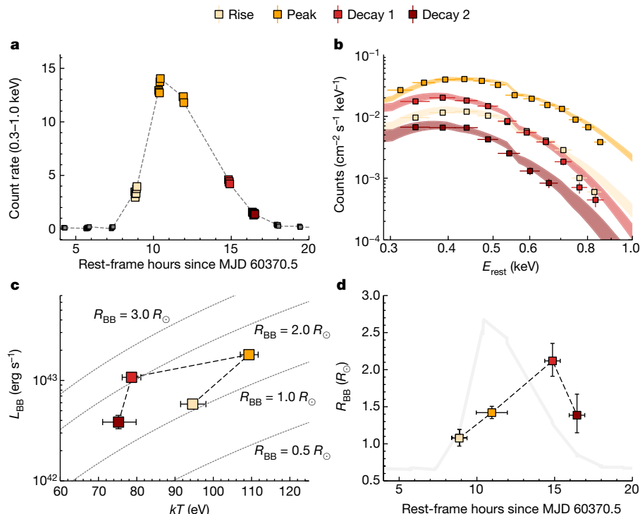
Fig. 2 | NICER time-resolved spectroscopy of the second eruption in Fig. 1b.
