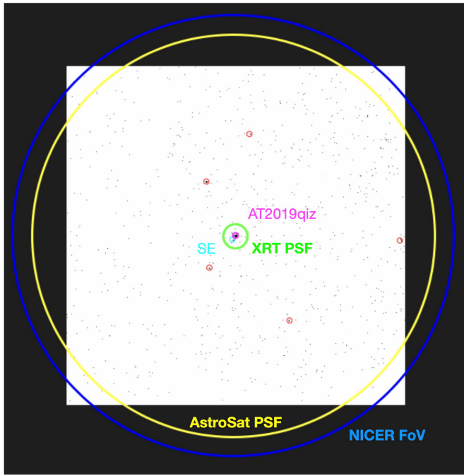
Extended Data Fig. 1 | Chandra image during eruption. The image is 8.5 \times 8.5 arcmin, with north up and east to the left. Five sources are detected within a few arcminutes of AT2019qiz. Only AT2019qiz shows statistical evidence of variability in the Chandra data (Methods). The PSFs (half-encircled energy width) of Swift/XRT and AstroSat are marked, as is the NICER field of view. None of the sources exhibit a count rate (0.3–1.0 keV) above about 10% of the count rate from AT2019qiz during eruption. Figure 1a shows a zoom-in of the central region.
