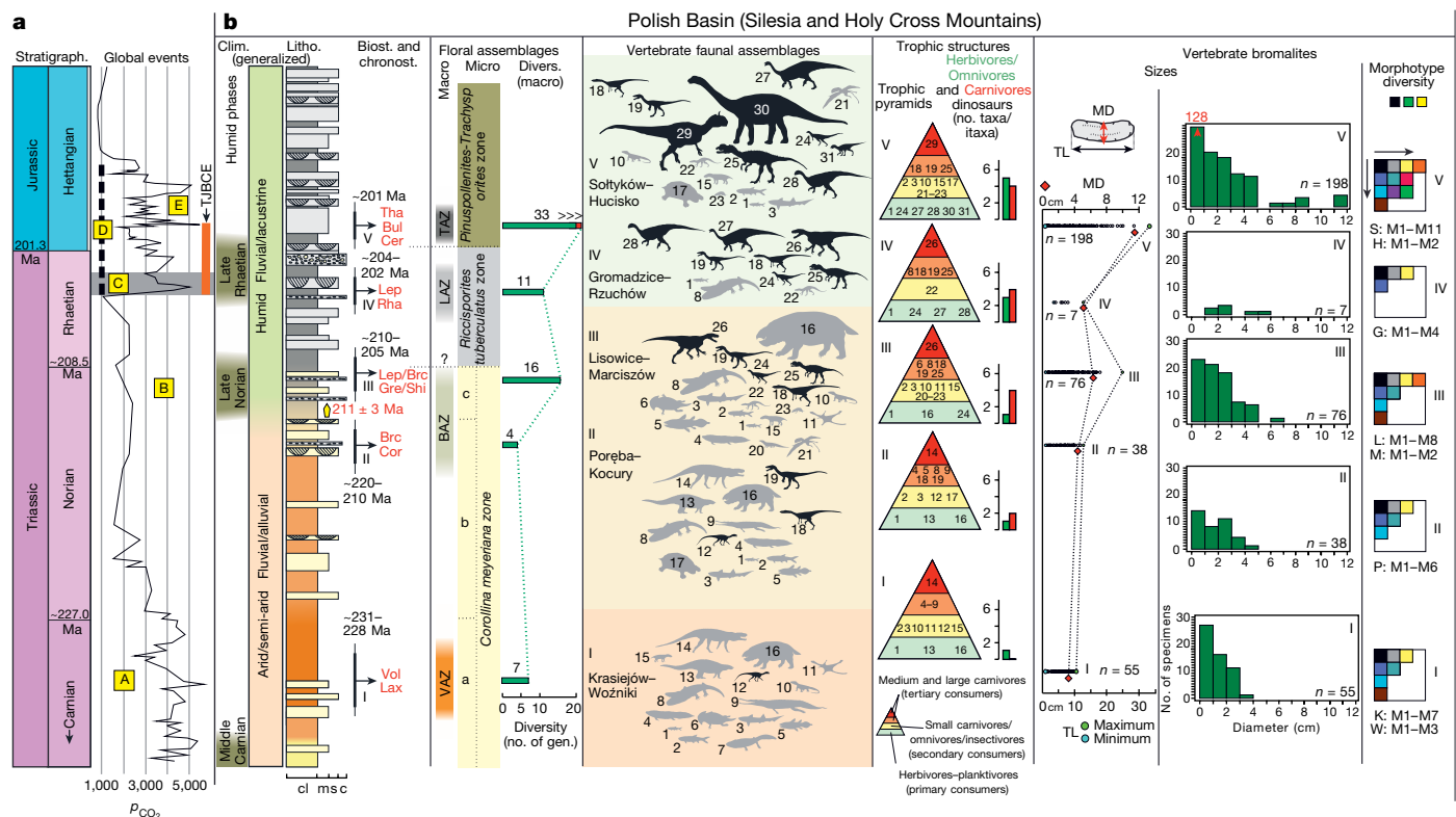
Fig. 1 | Terrestrial vertebrate assemblages from the Polish Basin across the Carnian to Hettangian. a , Global events: curve of partial pressure of CO 2 in ppm. A, oldest dinosaurs; B, the first phase of dinosaur radiation (late Norian); C, end-Triassic extinction; D, CAMP volcanism; E, the first ecosystems dominated by dinosaurs. b , Geological and fossil record from the Polish Basin. Clim., climatology; Litho., lithology; Biost., biostratigraphy; Chronost., chronostratigraphy; Divers., diversity; TJBCE, Triassic–Jurassic boundary climatic events in the Polish Basin 7 ; gen., genera; Vol, Voltzia flora; Lax, Laxitextella conchostracan fauna; Cor, Corollina meyeriana palynoflora; Brc, Brachyphyllum flora; Gre/Shi, Gregoriusella/Shipingia conchostracan fauna; Lep/Brc, Lepidopteris/Brachyphyllum flora; Lep, Lepidopteris flora; Rha, Rhaetipollis germanicus ; Cer, Cerebropollenites thiergartii ; Bul, Bulbilimnadia conchostracan fauna; Tha, Thaumatopteris flora; VAZ, Voltzia floral assemblage zone; BAZ, Brachyphyllum floral assemblage zone; LAZ, Lepidopteris floral assemblage zone; TAZ, Thaumatopteris floral assemblage zone. Vertebrate diversity (Supplementary Table 2): I–V, vertebrate assemblages (dinosauriforms represented by black and non-dinosauriform vertebrates by grey silhouettes).
