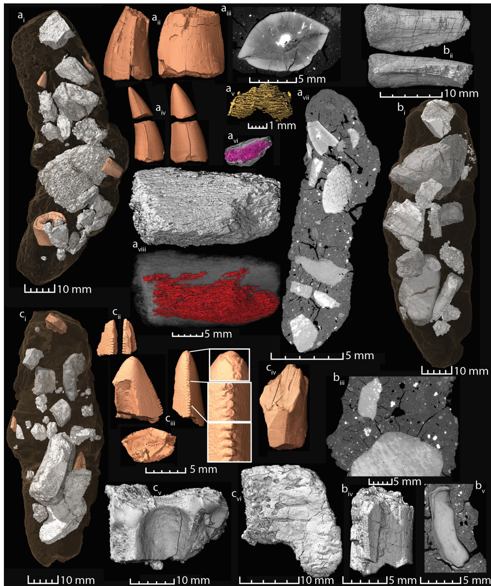
Extended Data Fig. 8 | Coprolites assigned to Smok wawelski (Lisowice).
