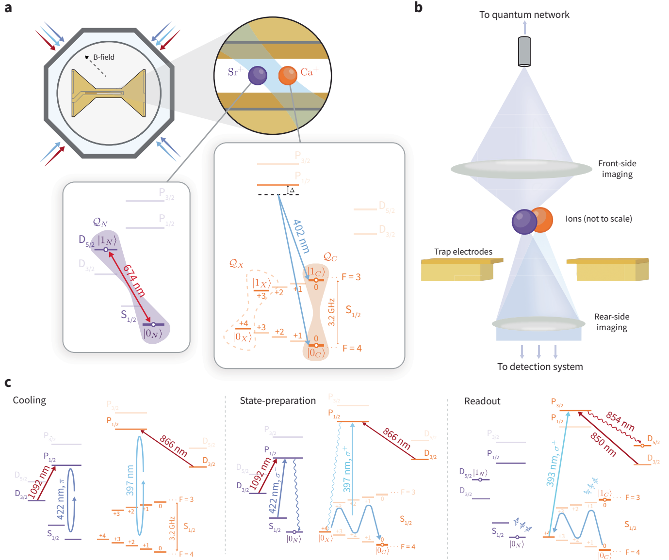
Extended Data Fig. 1 | Outline of a trapped-ion module. a , An ultrahigh-vacuum chamber houses a microfabricated surface Paul trap, which co-traps one ^{88}\text{Sr}^+ ion and one ^{43}\text{Ca}^+ ion. The ions are manipulated using lasers, which are delivered parallel to the surface of the trap. The \text{Sr}^+ ion provides an optical network qubit, Q_N , which is coherently manipulated using a 674-nm laser. The ground hyperfine manifold of the \text{Ca}^+ ion provides a circuit qubit, Q_C , and an auxiliary qubit, Q_X . The qubits in the ground hyperfine manifold are addressed using a pair of 402-nm Raman beams. b , The rear-side imaging system is used to perform fluorescence detection for qubit readout of both species. The front-side imaging system is used for single-photon collection from the \text{Sr}^+ ion during
