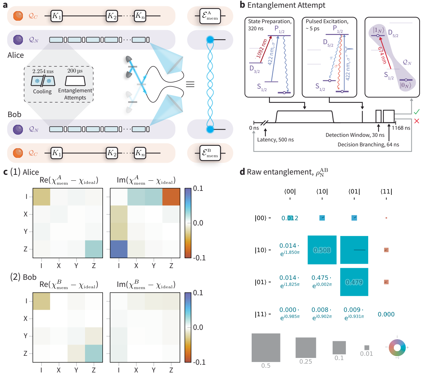
Extended Data Fig. 2 | Generation of remote entanglement and robust memory of the circuit qubits. a , Entanglement is generated between the network qubits using 200 \mu s of entanglement attempts interleaved with 2.254 ms of sympathetic recoupling using the \text{Sr}^+ ion. This is repeated until the entanglement is successfully heralded by a particular detector click pattern. While attempting to generate entanglement between the network qubits, Knill dynamical decoupling pulses, K_i , are used to preserve the state of the circuit qubits. b , Each entanglement attempt has a total duration of 1168 ns. We perform a 320-ns state-preparation pulse (which has a switching latency of 500 ns), pumping the \text{Sr}^+ ion into the lower ground Zeeman state. An approximately 5-ps pulse excites the \text{Sr}^+ ion to the upper P_{1/2} level (lifetime about 7 ns), which rapidly decays to one of the ground Zeeman levels, thereby generating ion-photon entanglement. We collect a photon from each of the modules, interfere
