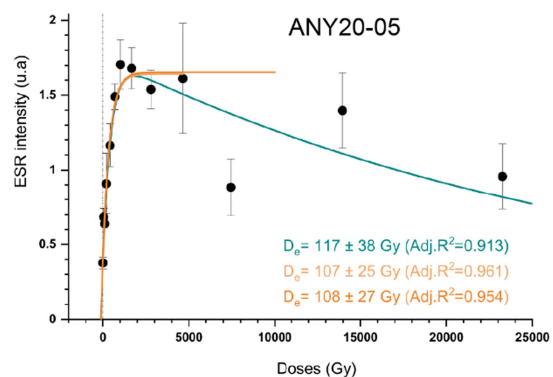
Extended Data Fig. 5 | ESR dose response curves (DRCs) derived from the Ti-H ESR signal measured in the quartz samples from Bété I. Fitting was performed as follows: (see text for further information): a , with the Ti-2 function (data weighting by 1/s^2 ); b , with the single saturating exponential (SSE) function (data weighting by 1/l^2 ) with D_{max} = 4.5 kGy; and c , D_{max} = 2.8 kGy.
