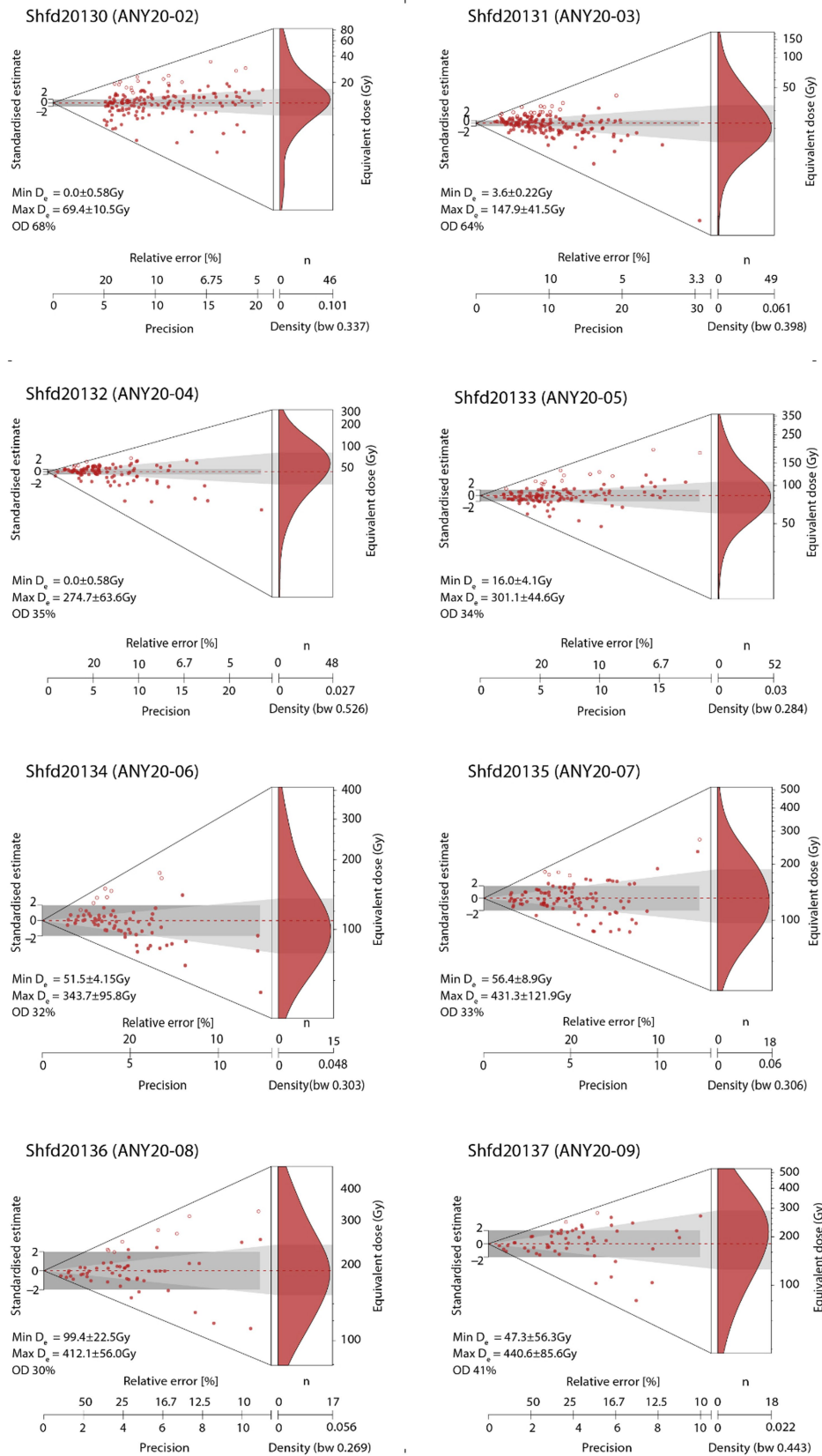
Extended Data Fig. 6 | Abanico plots of D_e replicate single grain (SG) OSL data centred on the Central Age Model D_e also used for age calculation purposes. Open circles indicate aliquots considered as outliers (see SI-3 for
