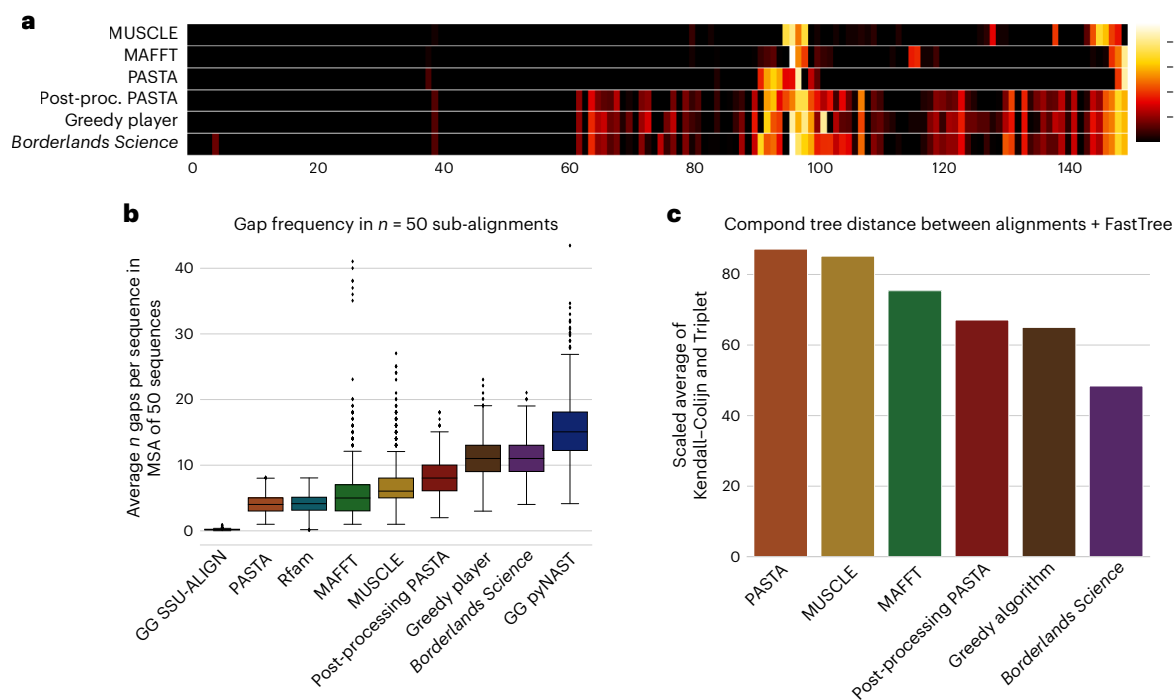
Fig. 2 | Evaluation of the alignment. a , Here the gap density by column is shown for six different alignment methods. The x axis corresponds to the alignment position, and the color corresponds to the log gap frequency at this position. Highly gapped columns were excluded so all alignments could be of the same length. b , Gap frequencies observed in BLS and other methods, averaged from sampled sub-alignments of 50 sequences. The box plot shows an overview of the distribution. The three horizontal lines in the box, from top to bottom, show, respectively, the boundaries for the upper quartile, the middle quartile
